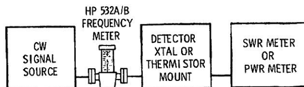
Figure 1. Typical Frequency-Measuring Setup
