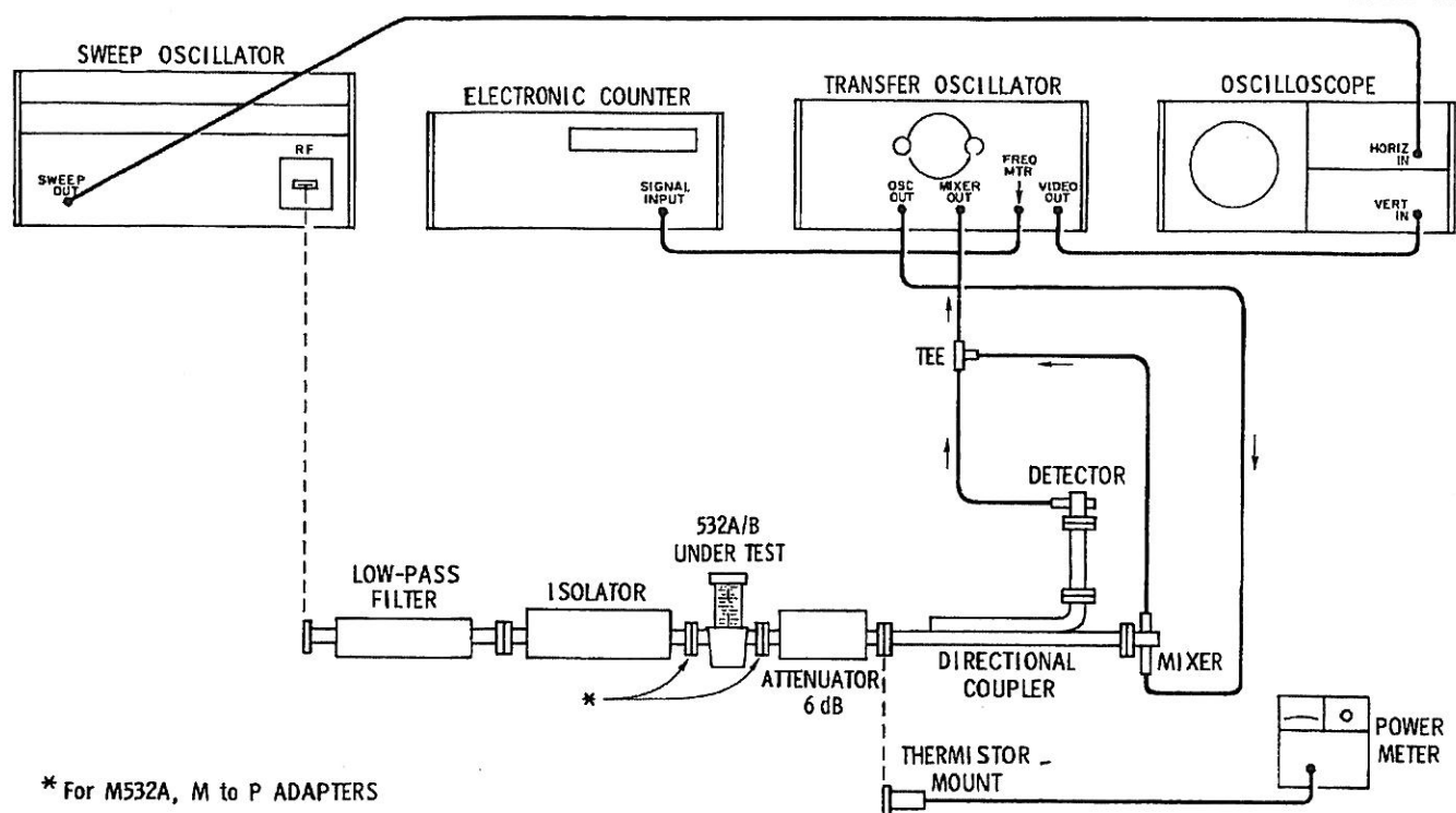
FIGURE 3. PERFORMANCE TEST
