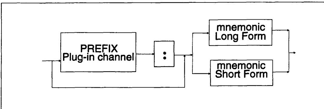
Figure 2.2: Command Header
