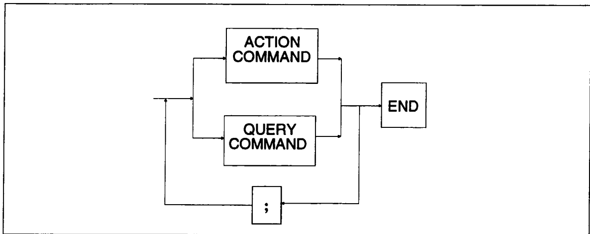
Figure 2.6: Multiple Commands
