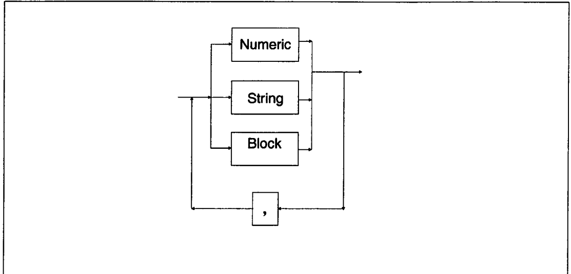
Figure 2.4: Command Arguments
