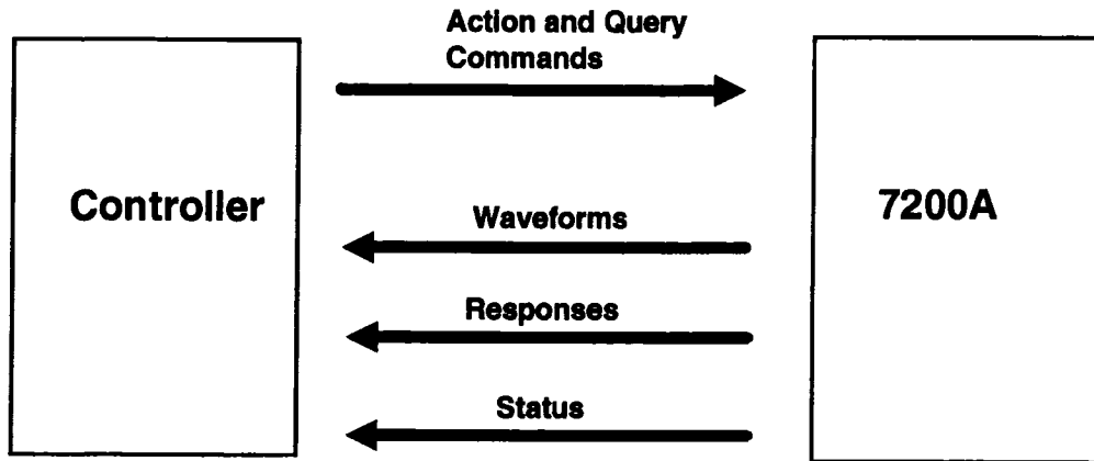
Figure 2.1: Message Directions
