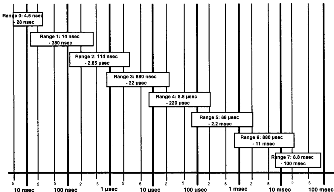
9215 Transition Time Ranges
