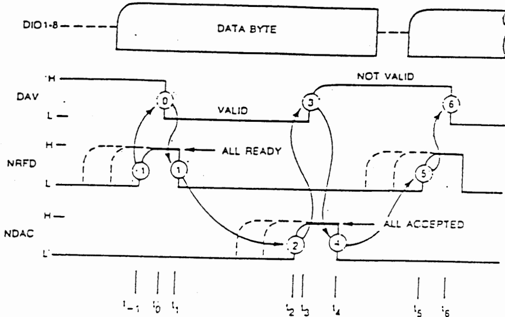
Figure 10.1 : DATA BYTE TRANSFER IN GPIB IEEE-488
