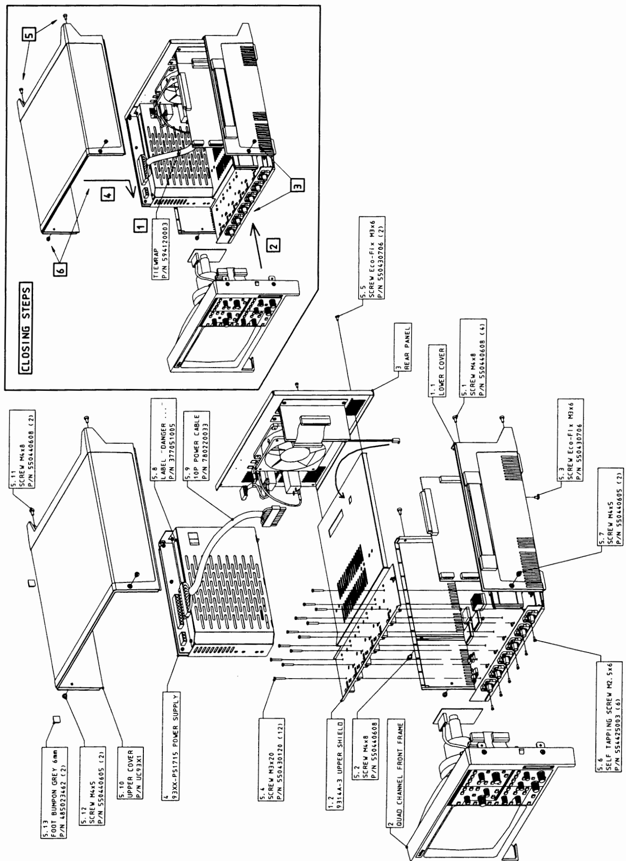
Figure 7.1 : 9314A/M/L Assembly
