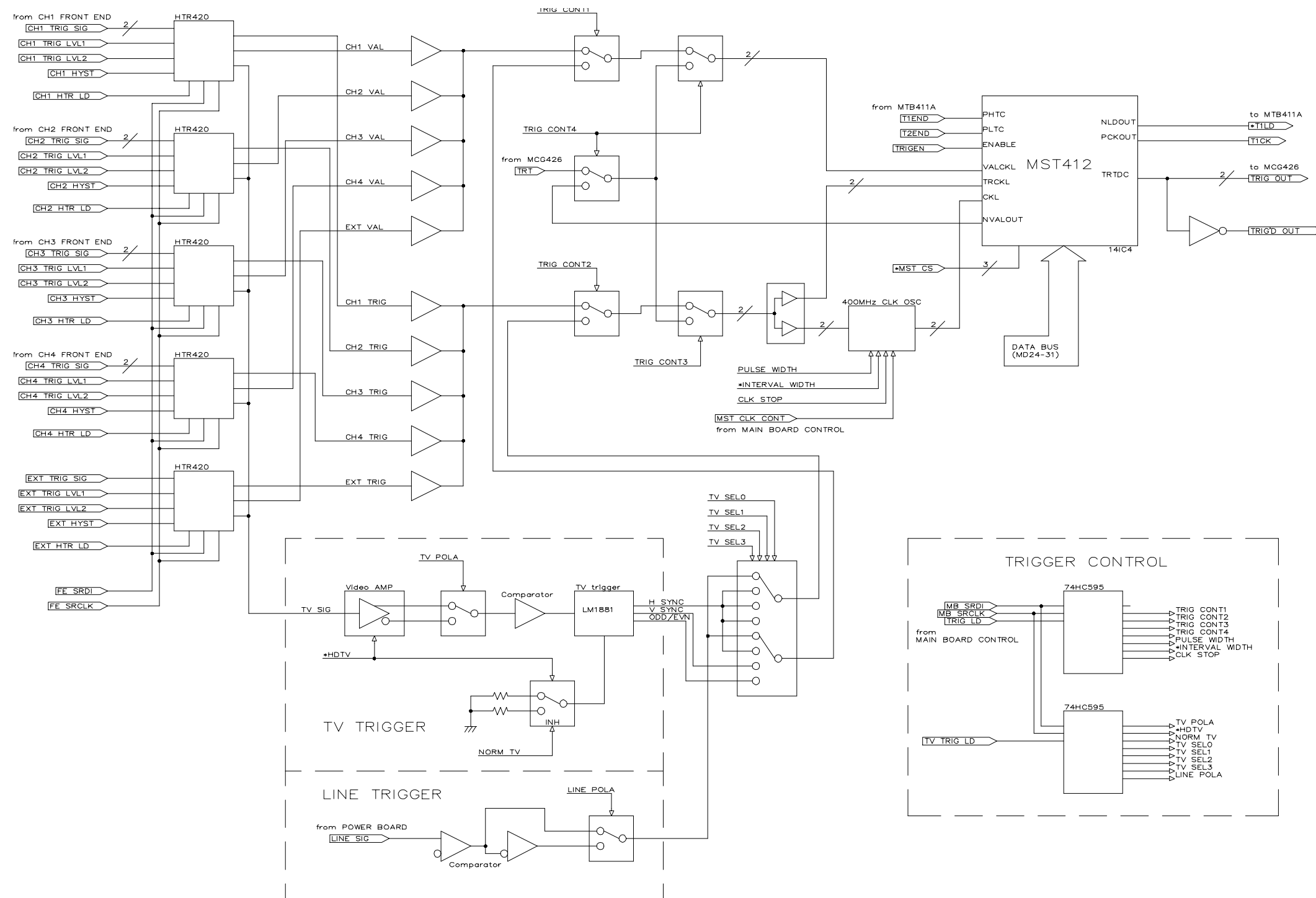
TRIGGER Block Diagram
