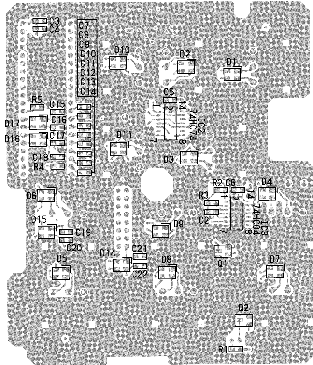
PANEL BOARD (2/2)
