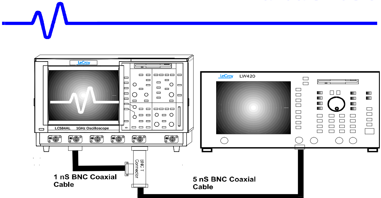
Figure 5-7 : External Trigger Equipment Setup
