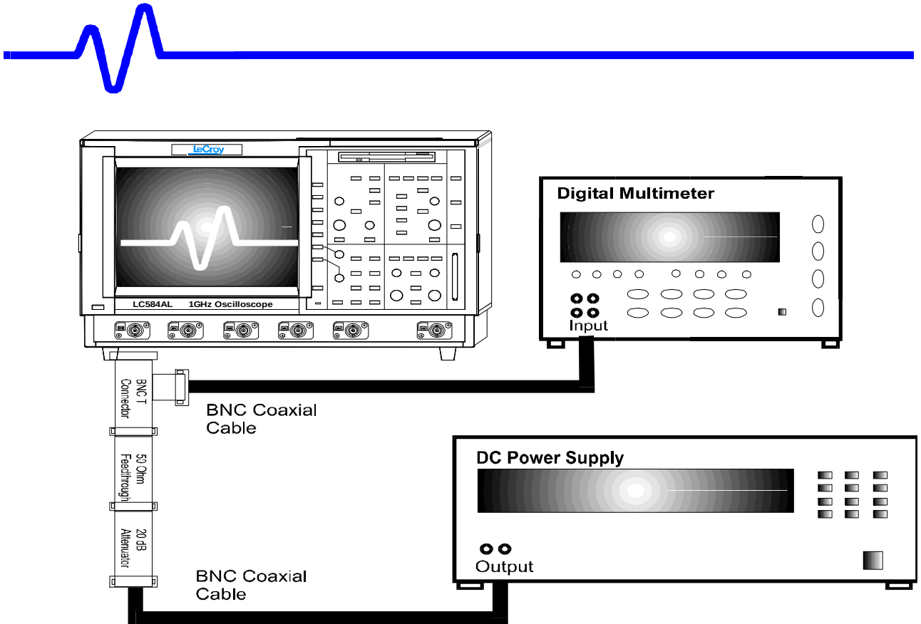
Figure 5-2 : DC 1MW Accuracy Equipment Setup for 100 mV/div
