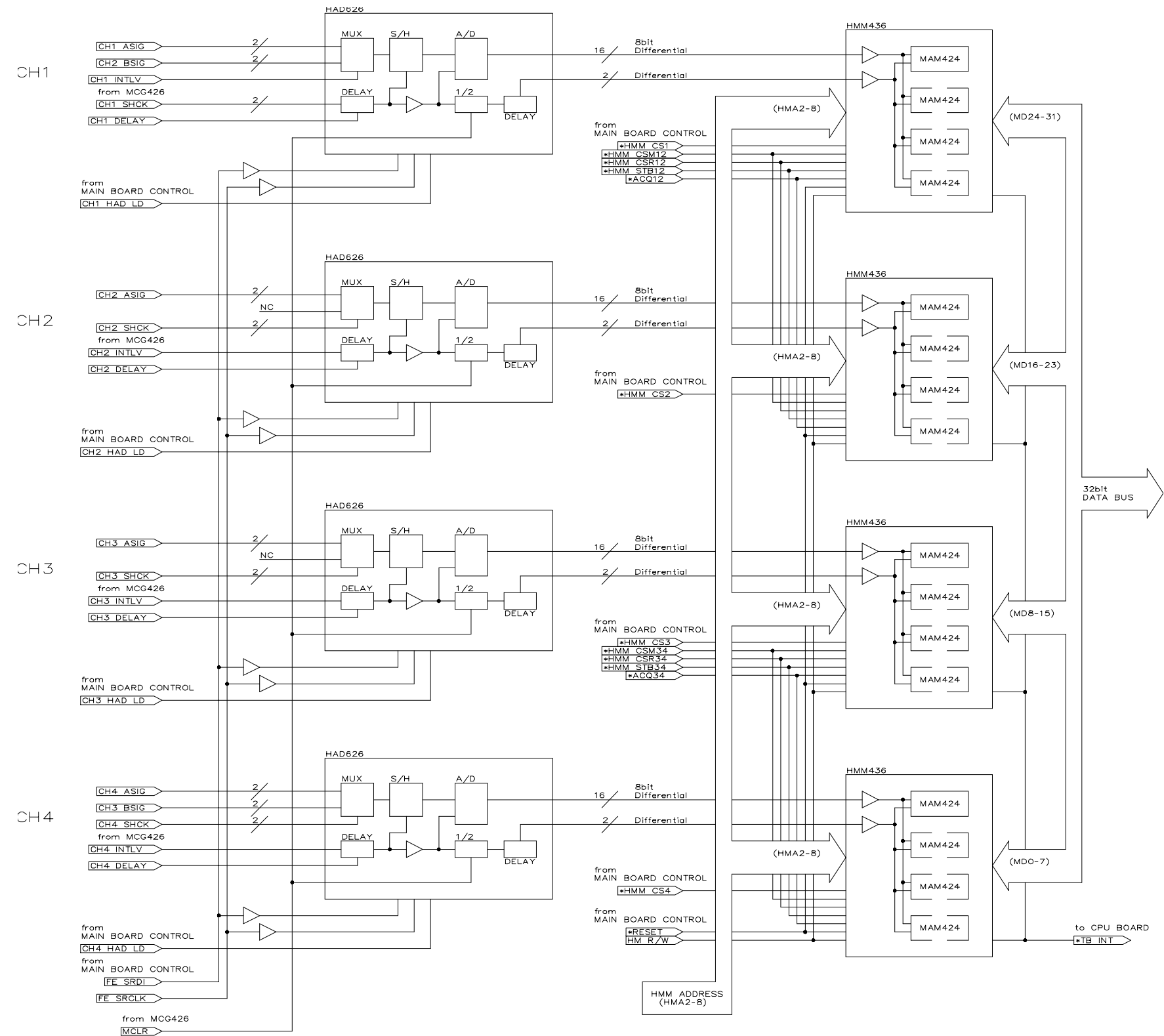
A/D CONVERTER & MEMORY Block Diagram
