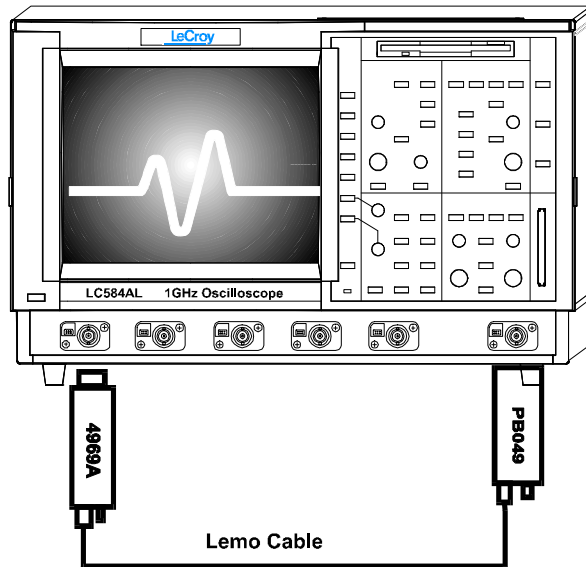
Figure 5-8: 50 W Overshoot & Rise time Equipment Setup
