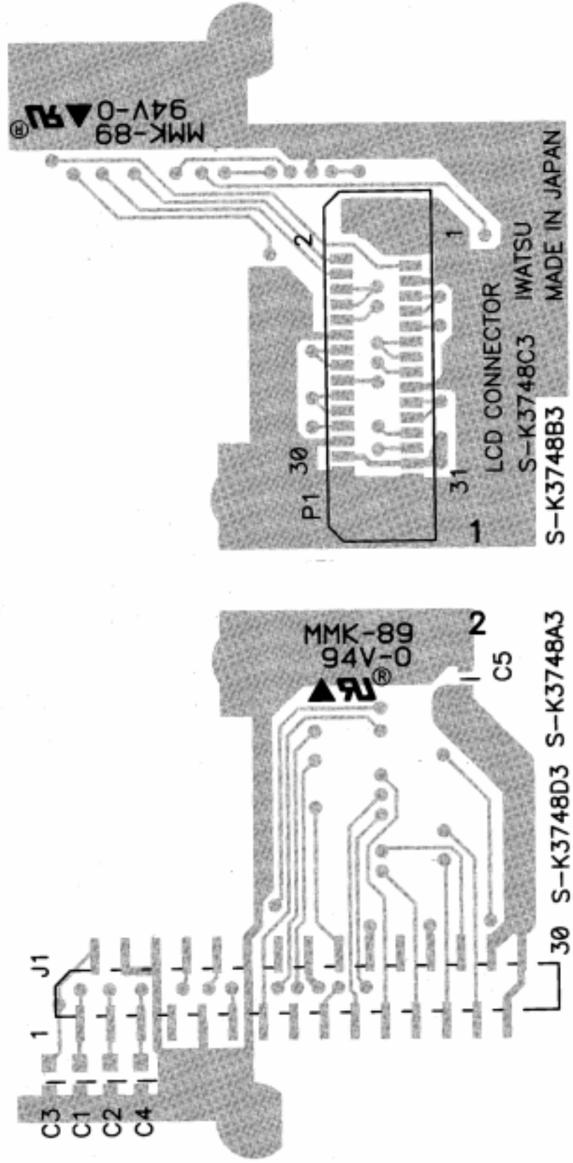
LCD CONNECTOR
