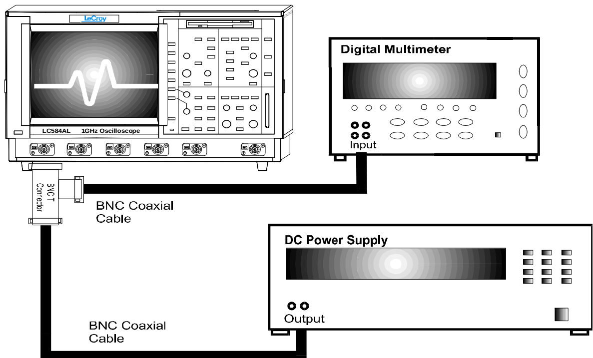
Figure 5-3 : DC 1MW Accuracy Equipment Setup for 5V/div.
