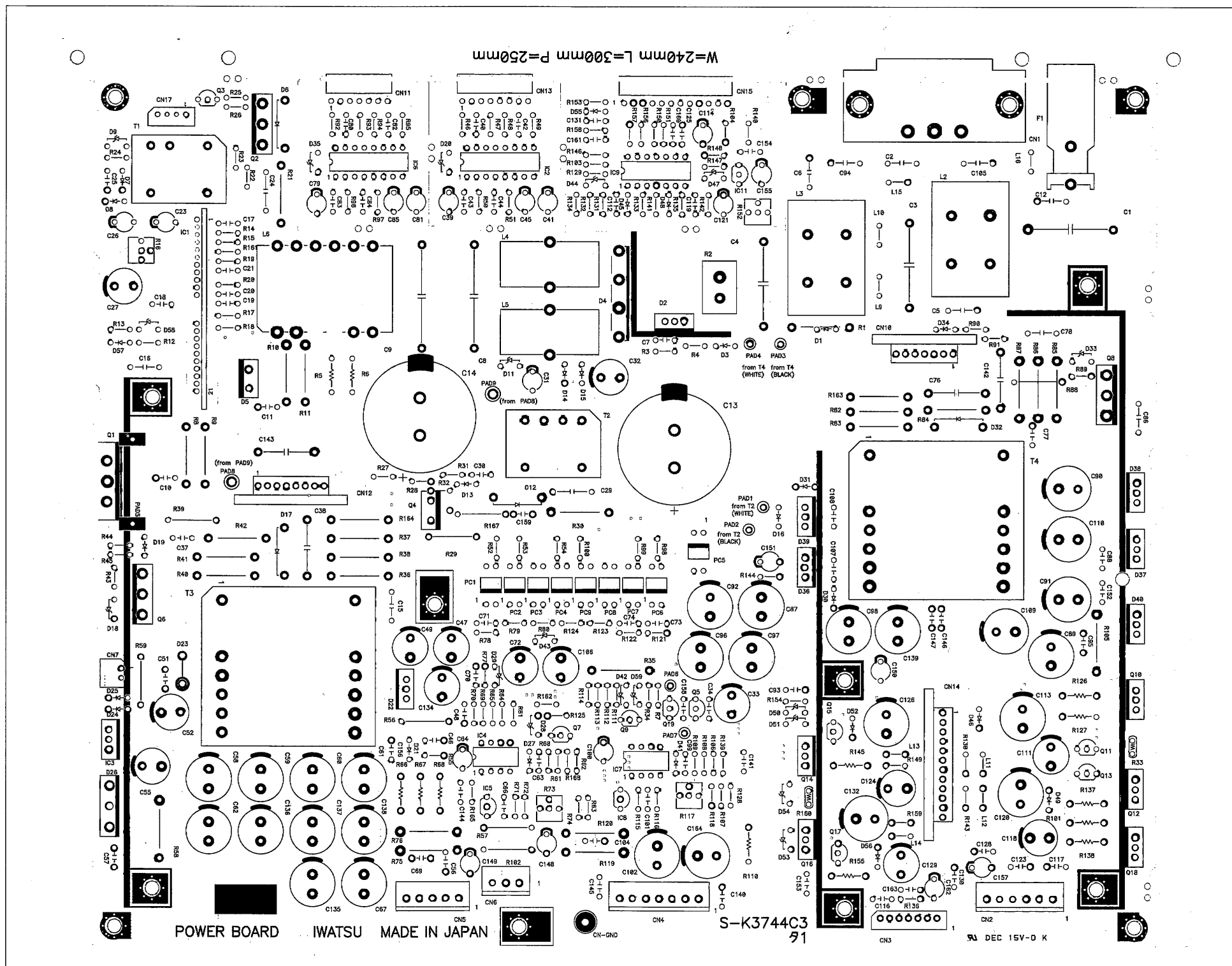
POWER BOARD
