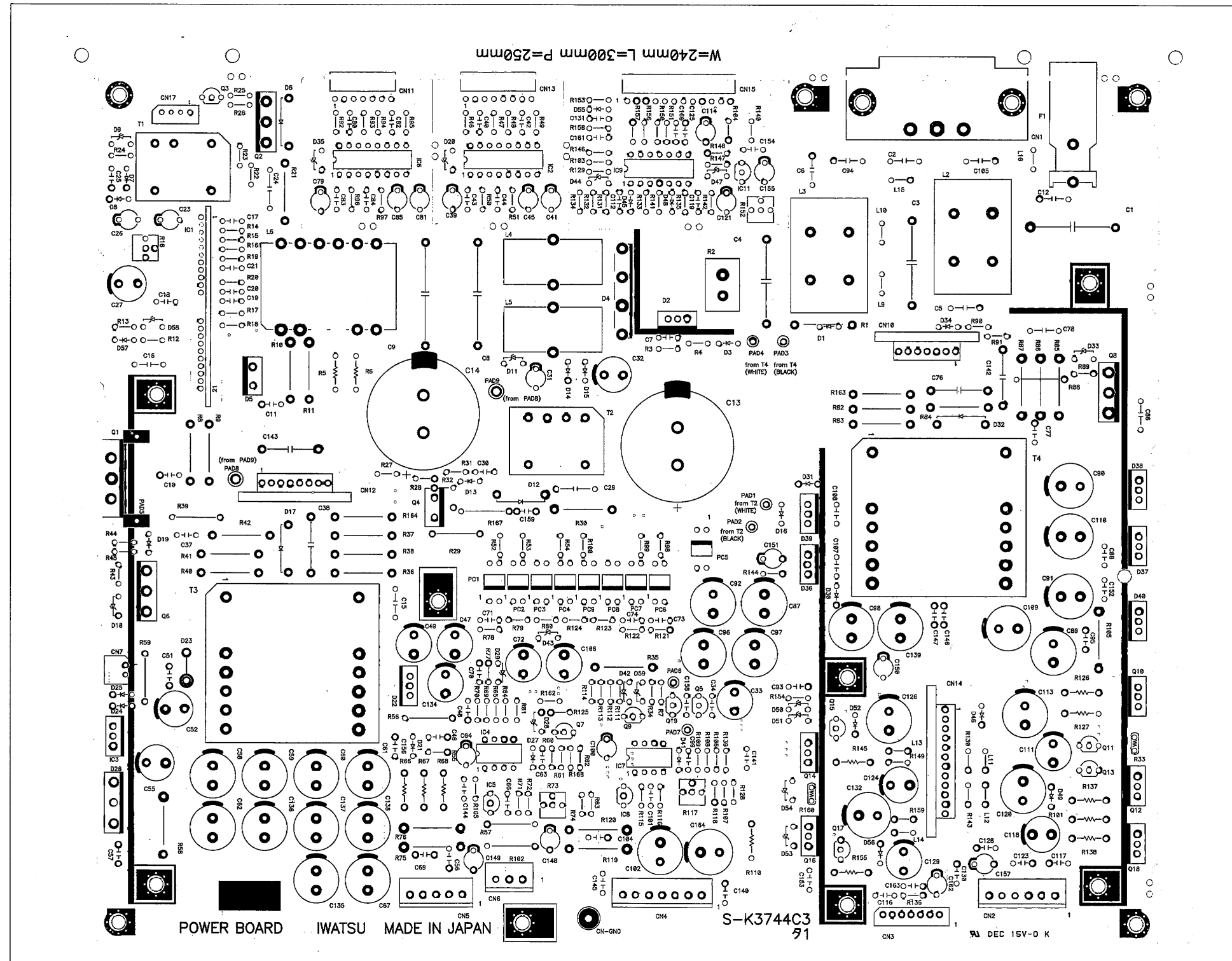
POWER BOARD
