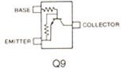
DTC114EU (Symbol: 24)
