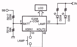
Fig. 11 Battery voltage detector and lamp circuits
