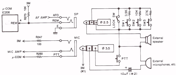
The voltage at the REM pin is normally about 3.5 V as a result of R273. When a remote control microphone button is pressed, this voltage is divided by the resistor connected in series with the button switch and by R273. The resulting voltage indicates which button was pressed.
