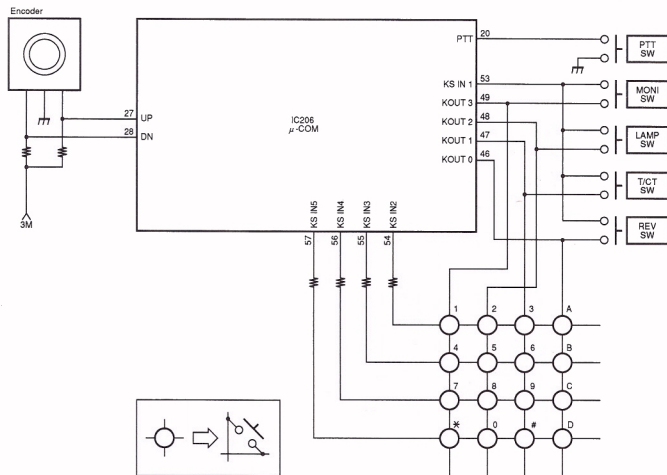
Fig. 9 Keys and rotary encoder circuit
