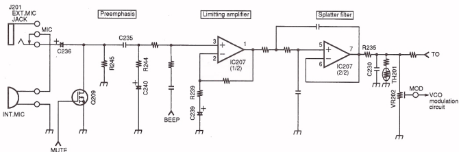
Fig. 5 Microphone amplifier
