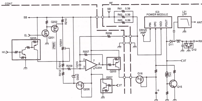
Fig. 6 APC and transmission output selector circuits
