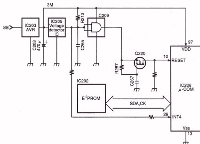
Fig. 10 Reset and backup circuits
