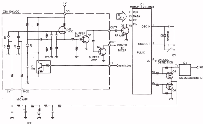
Fig. 7 PLL and VCO circuits
