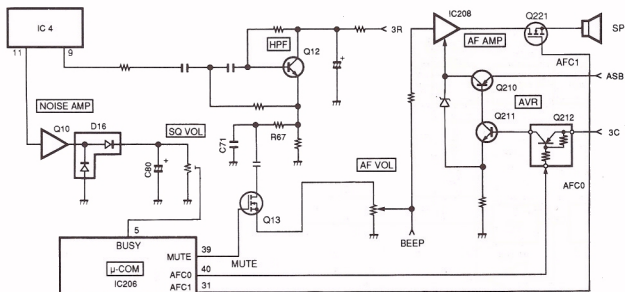
Fig. 3 AF amplifier, squelch, and mute circuits
