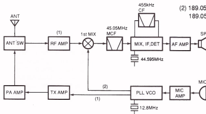
Fig. 1 Frequency configuration
