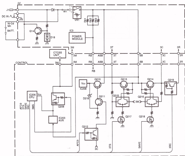
Fig. 12 Power supply circuit
