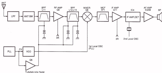
Fig. 2 Receiver section configuration
