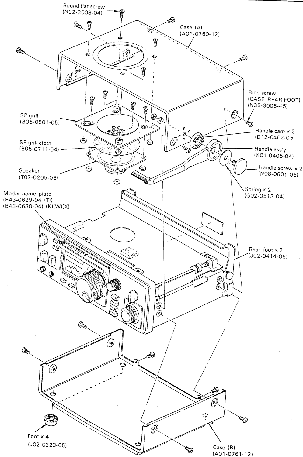
Fig. 3 Case disassembly
