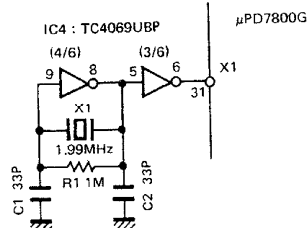
Fig. 15 System clock oscillation circuit
