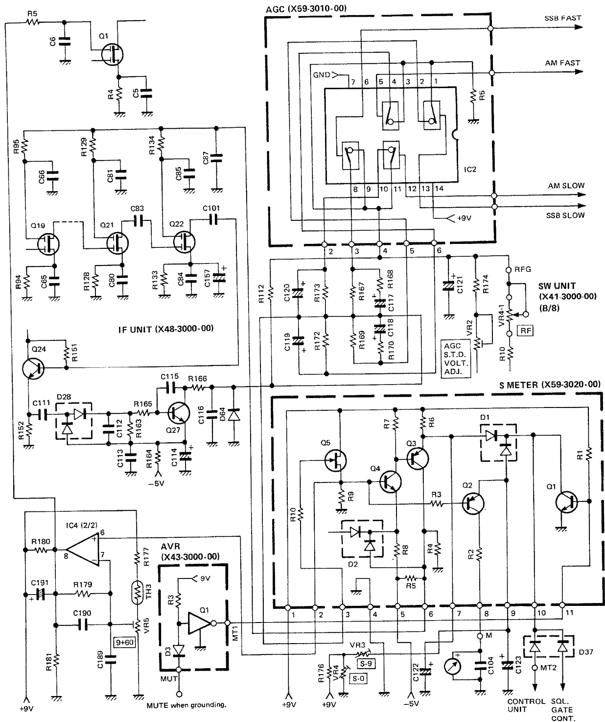
Fig. 8 AGC circuit
