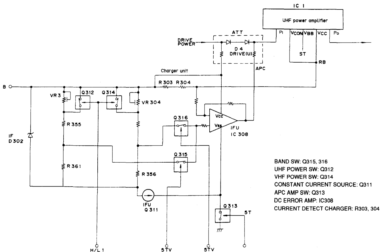
Fig. 6 APC operation
