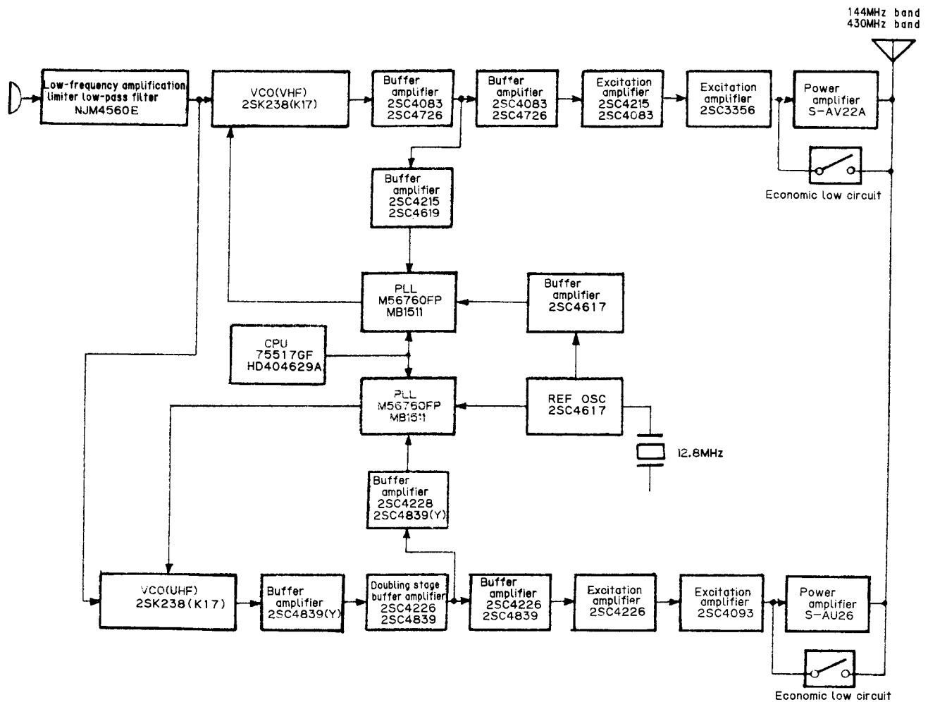
Fig. 5 Transmitter system
