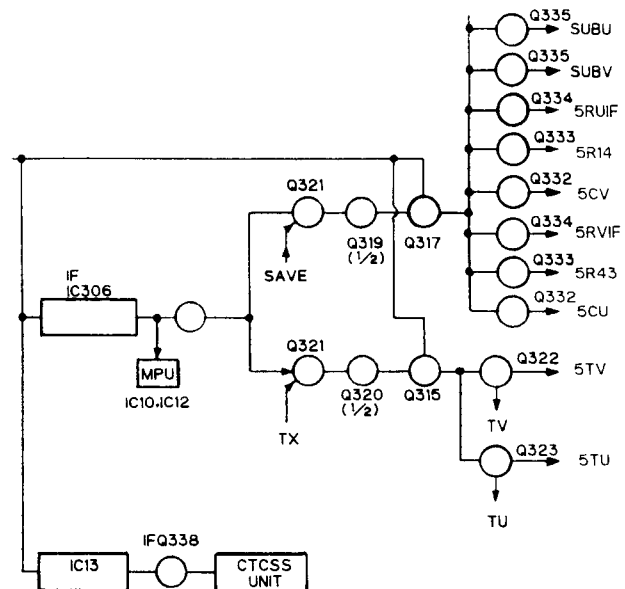
Fig. 7 Power supply circuit
