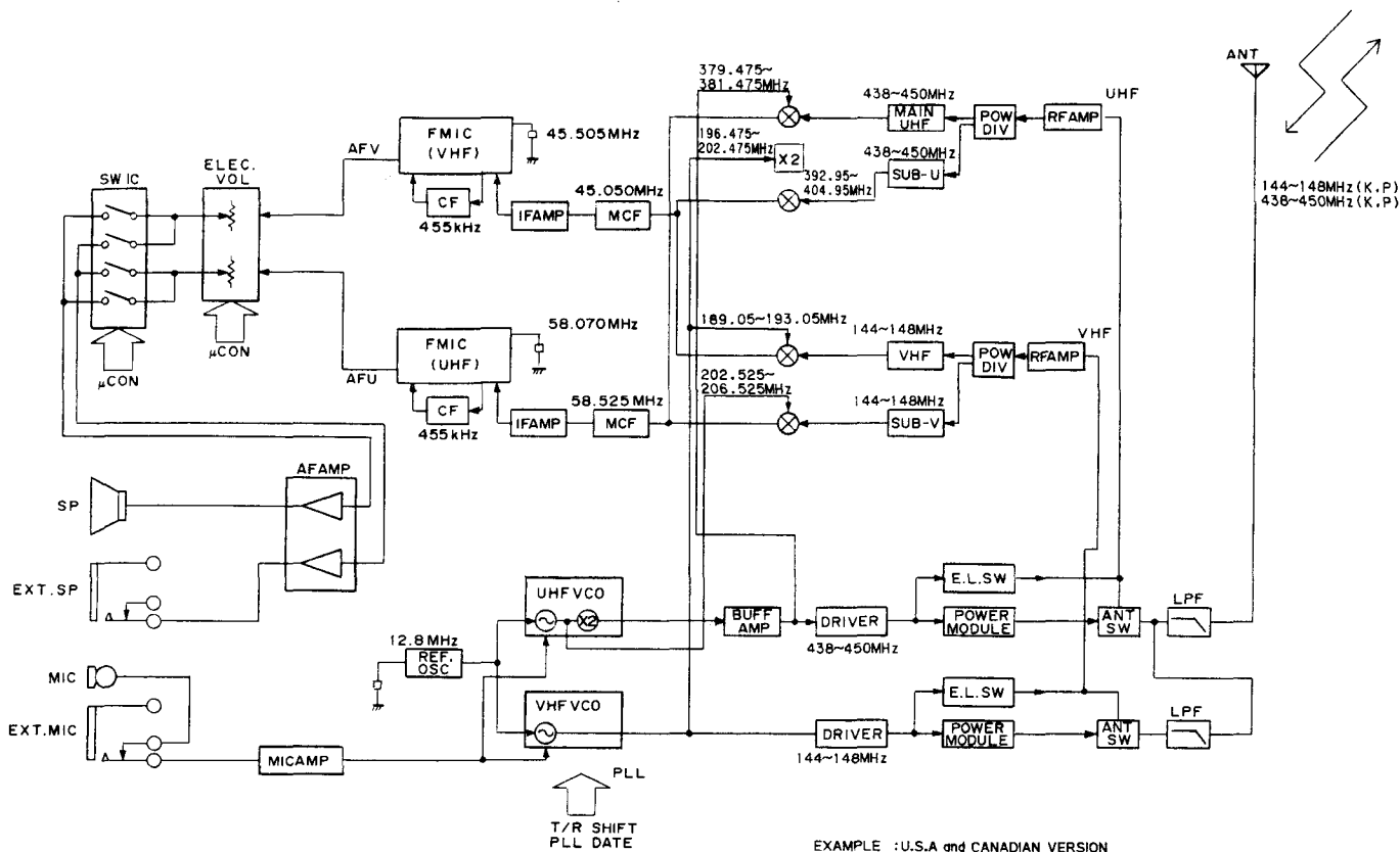
Fig. 1 Circuit configuration by frequency
