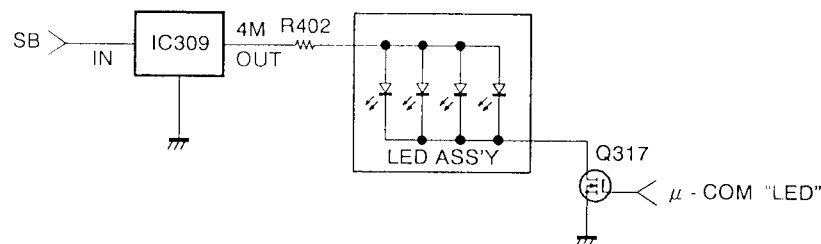
Fig. 11 LCD illumination
