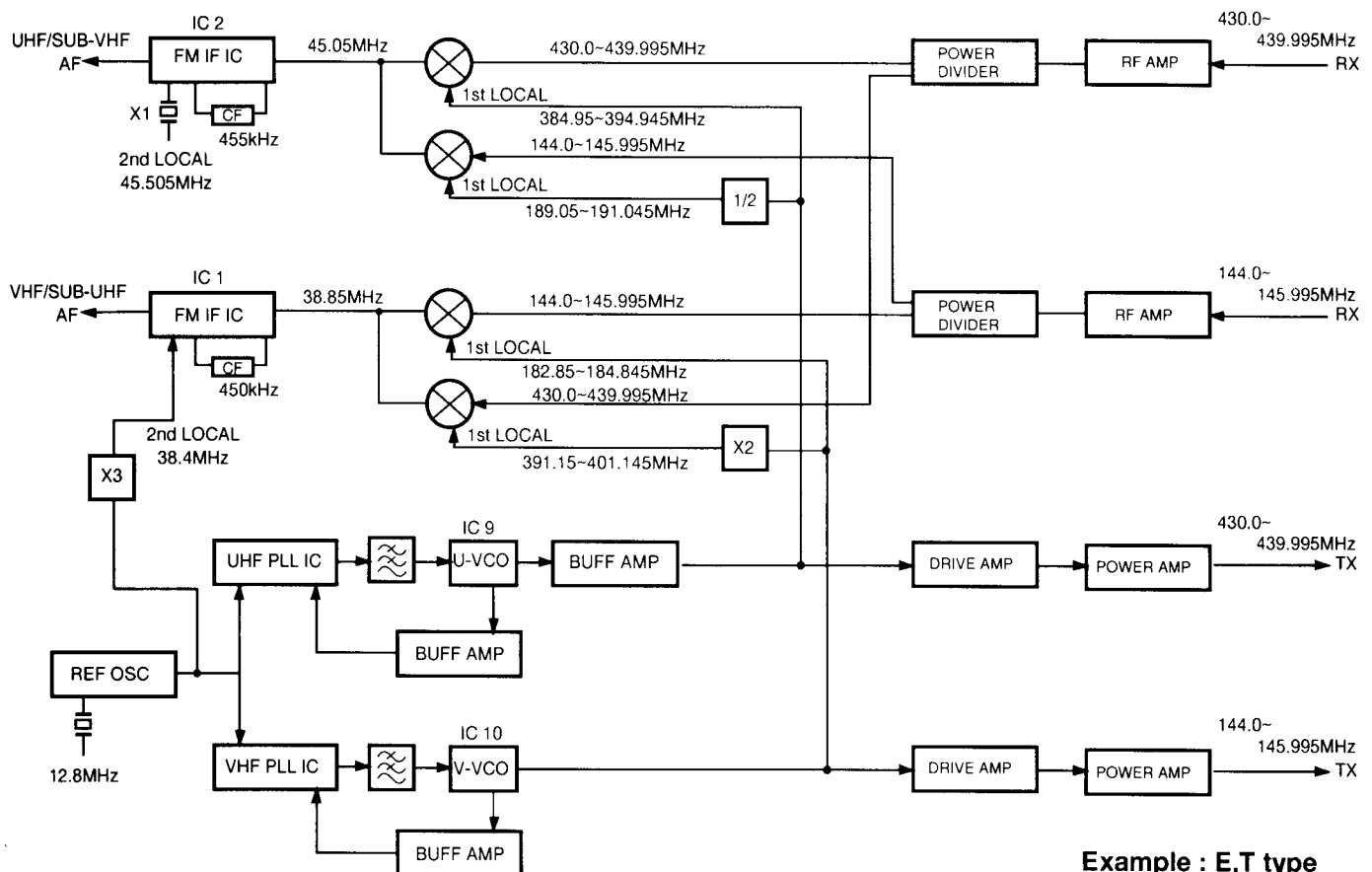
Fig.1 Frequency configuration
