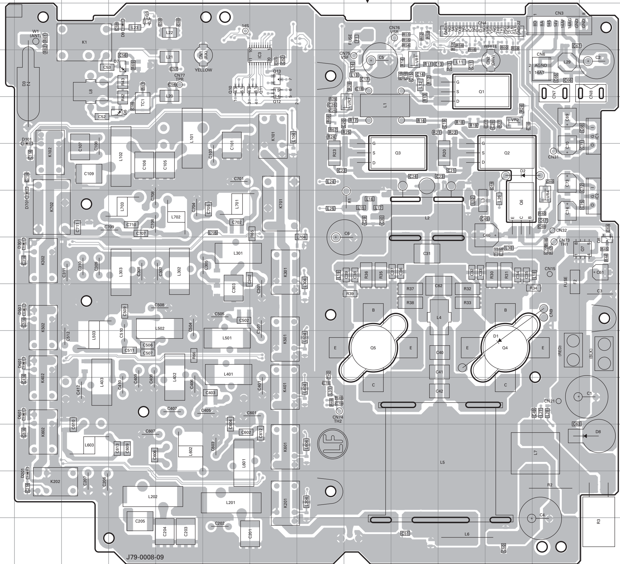
FINAL UNIT (X45-3780-20) Component side view (J79-0008-09)
