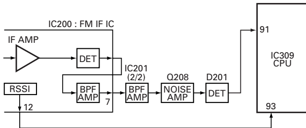
Fig. 5 Squelch circuit
