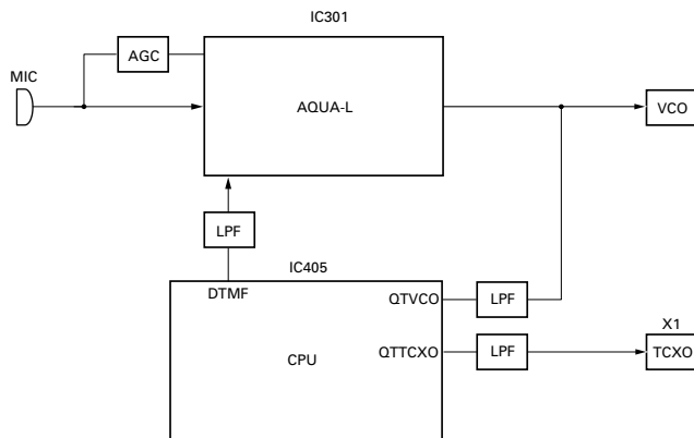
Fig. 6 Microphone amplifier
