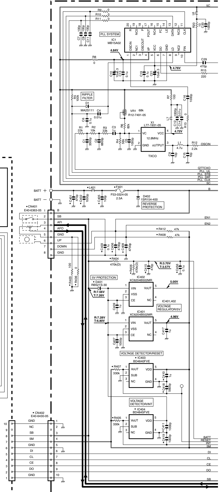
TX-RX UNIT (X57-7120-XX)
