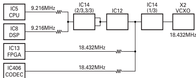
Fig. 10 Clock diagram
