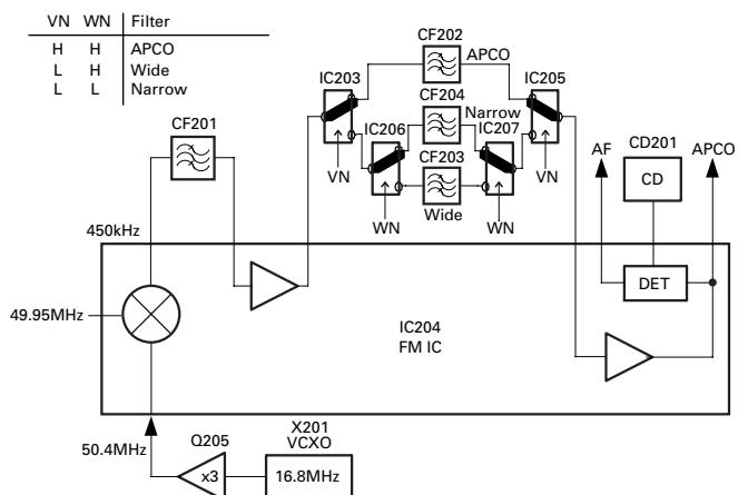
Fig. 3 Wide/Narrow/APCO switching circuit
