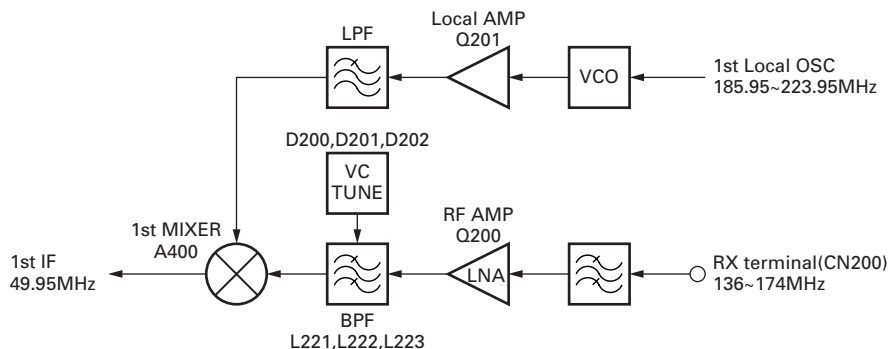
Fig. 2 Front-end RF amplifier and 1st local
