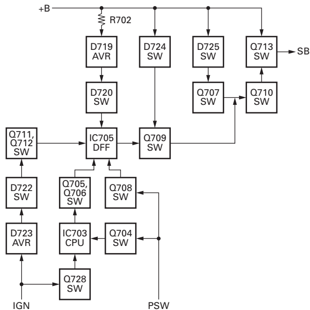
Fig. 14 Power supply circuit
