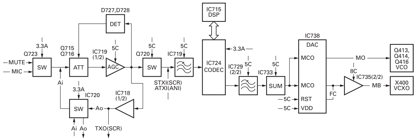
Fig. 7 Audio band and Base band circuit
