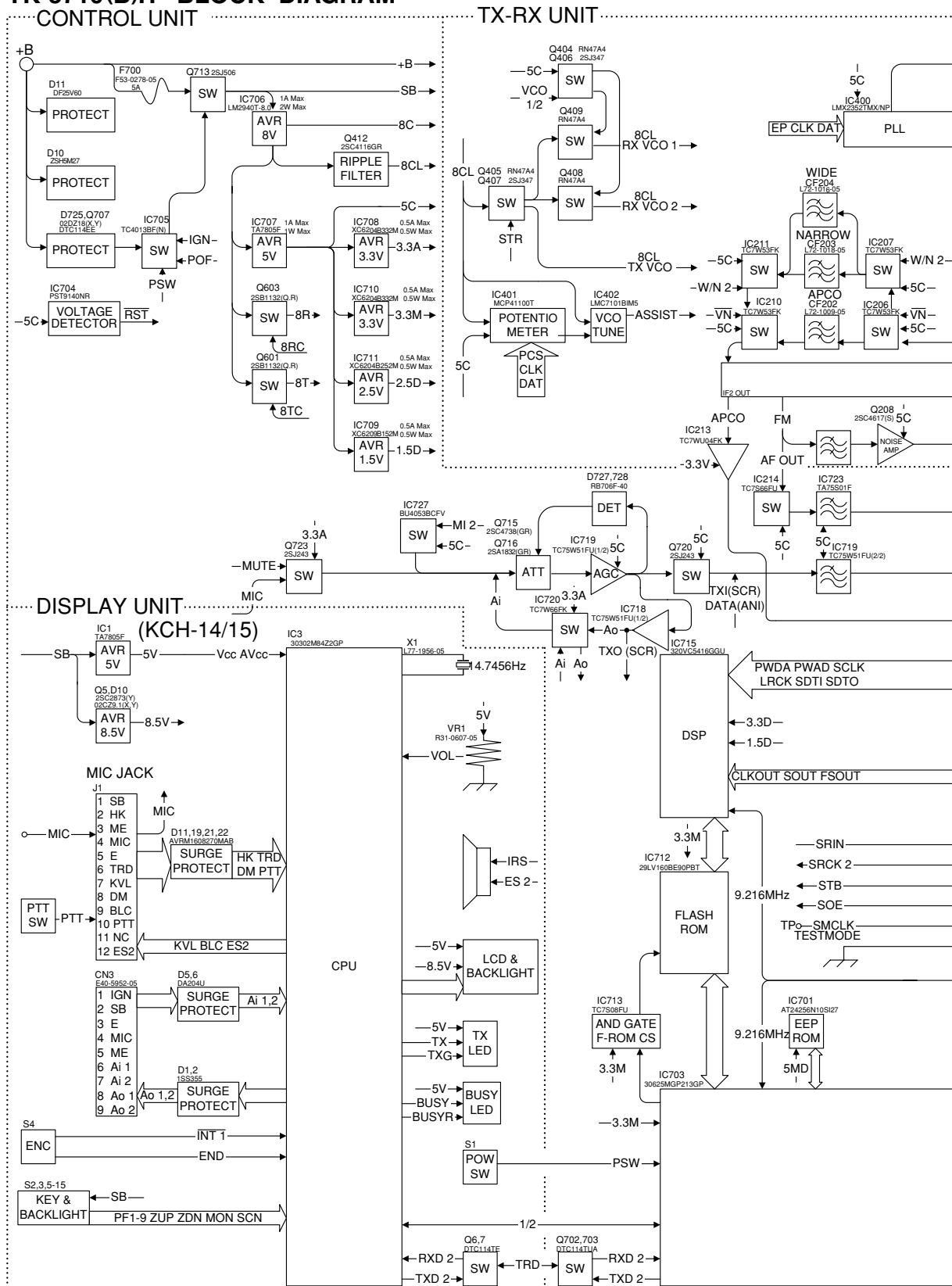
TK-5710(B)H BLOCK DIAGRAM
