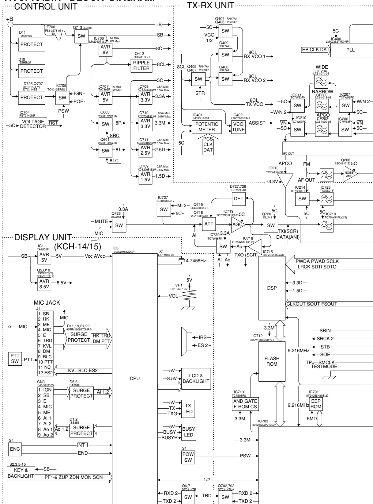
TK-5710(B)H BLOCK DIAGRAM
