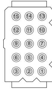
Figure 1-2 15-pin connector
