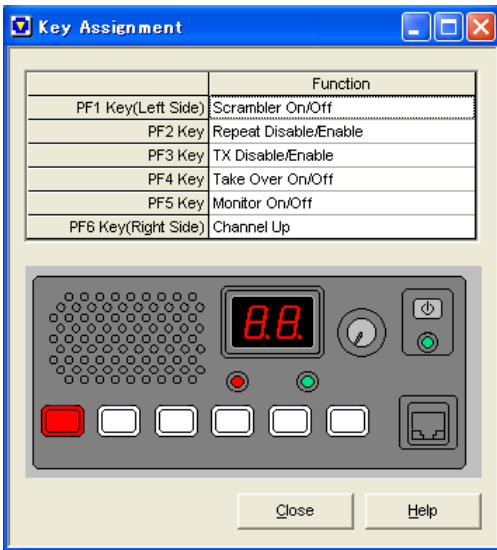
Figure 3-5 Key Assignment
