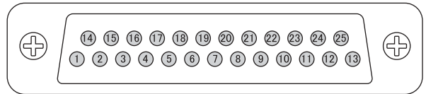
Figure 1-4 25-pin connector (D-SUB)
