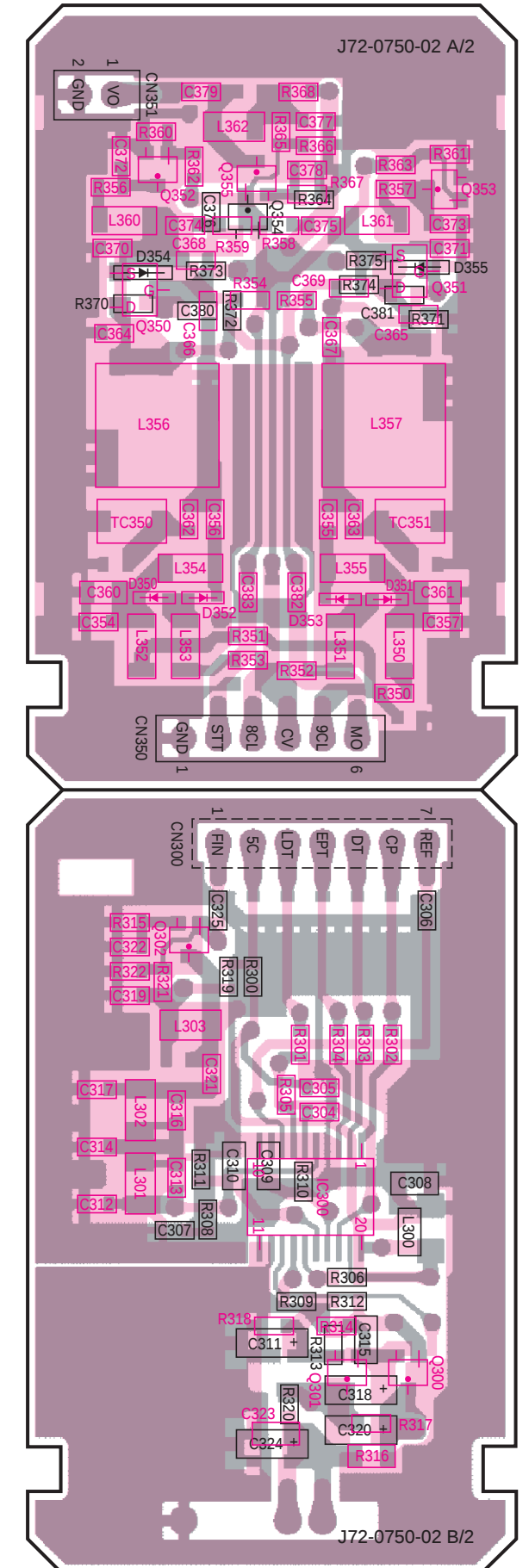
TX PLL/VCO (X58-4790-10) Foil side view
