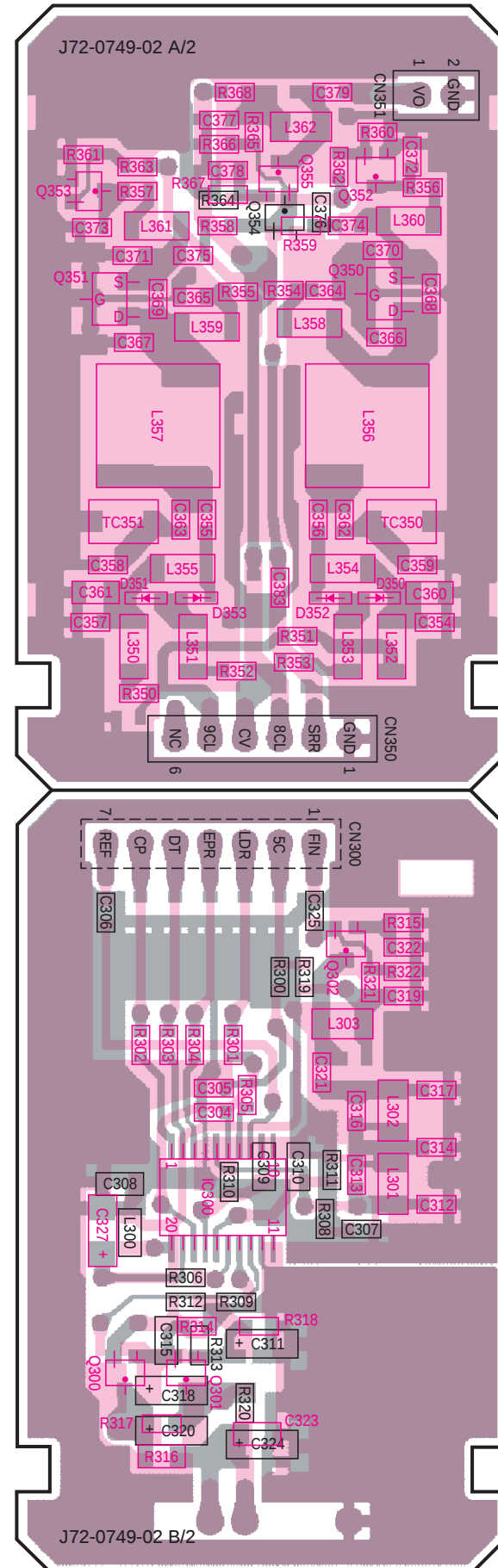
RX PLL/VCO (X58-4780-10) Component side view
