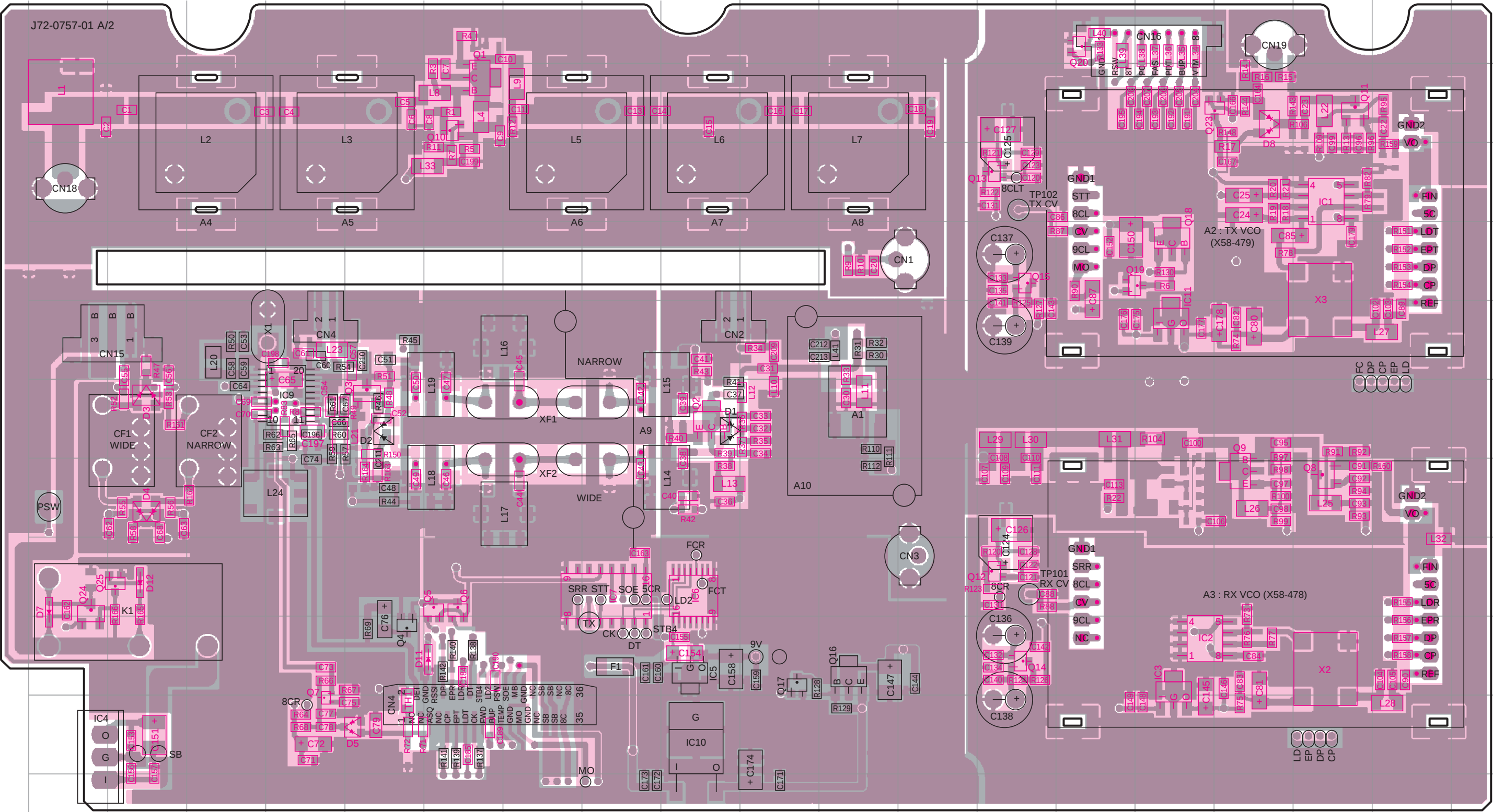
TX-RX UNIT (X57-6260-XX) (A/2) -10 : K,E -11 : K2 Component side view + Foil side
