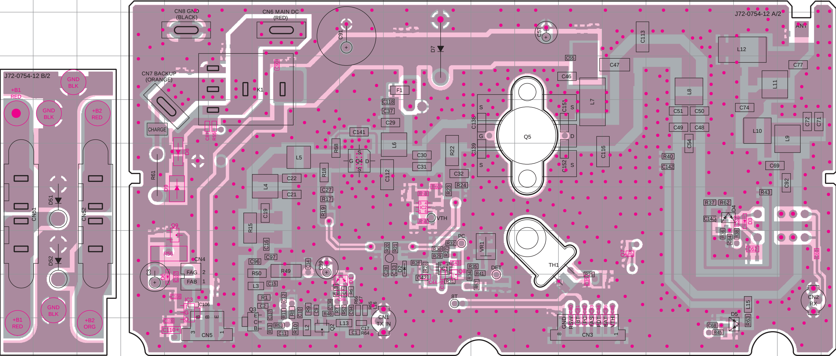
FINAL UNIT (X45-3620-XX) -10 : K,E -11 : K2 Component side view + Foil side
