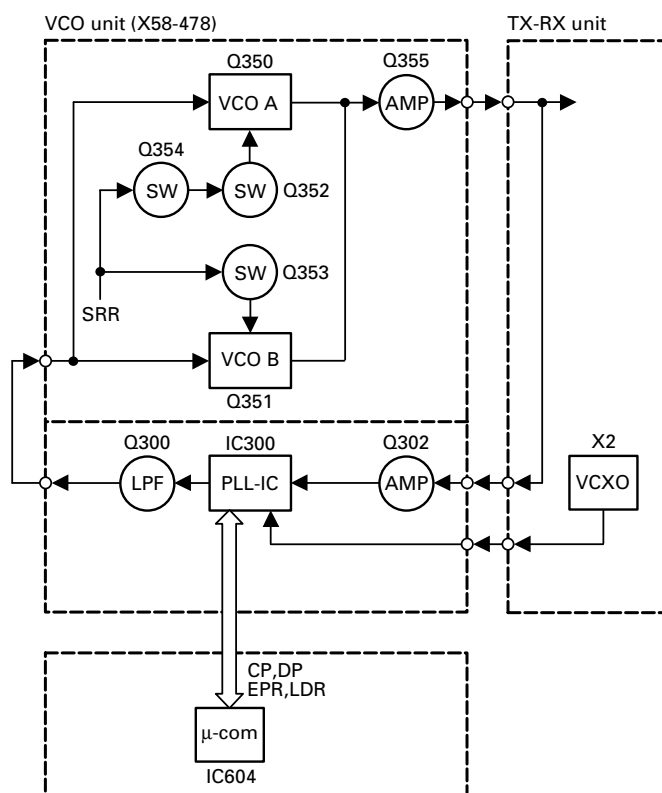
Fig. 5 Receiver PLL
