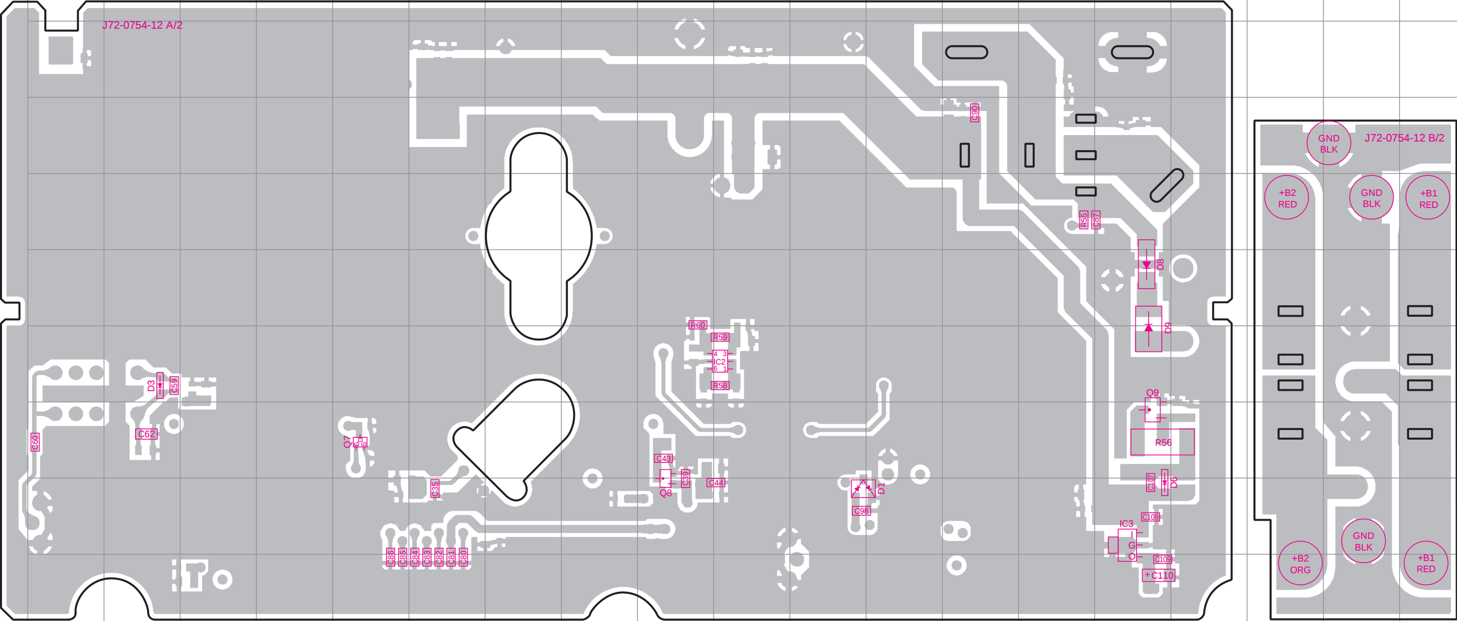
FINAL UNIT (X45-3620-XX) -10 : K,E -11 : K2 Foil side view
