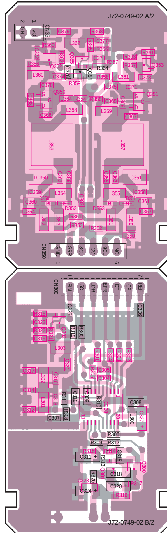
RX PLL/VCO (X58-4780-10) Foil side view
