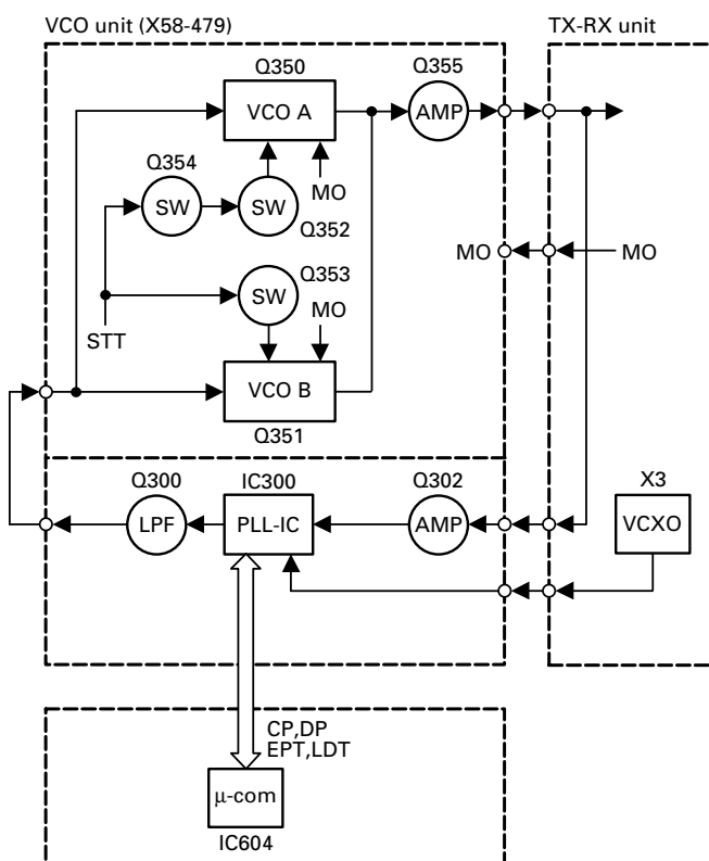
Fig. 6 Transmitter PLL
