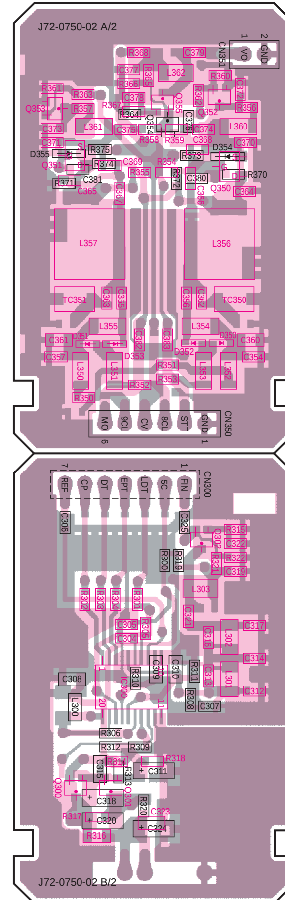
TX PLL/VCO (X58-4790-10) Component side view
