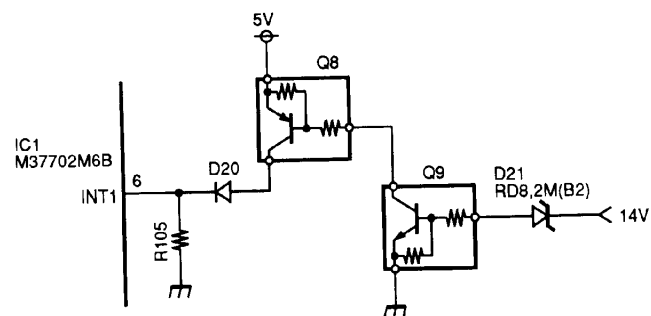
Fig. 18 Backup circuit
