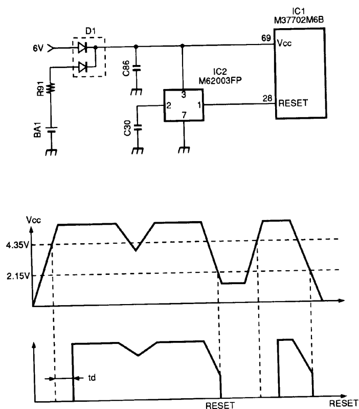
Fig. 17 Reset circuit
