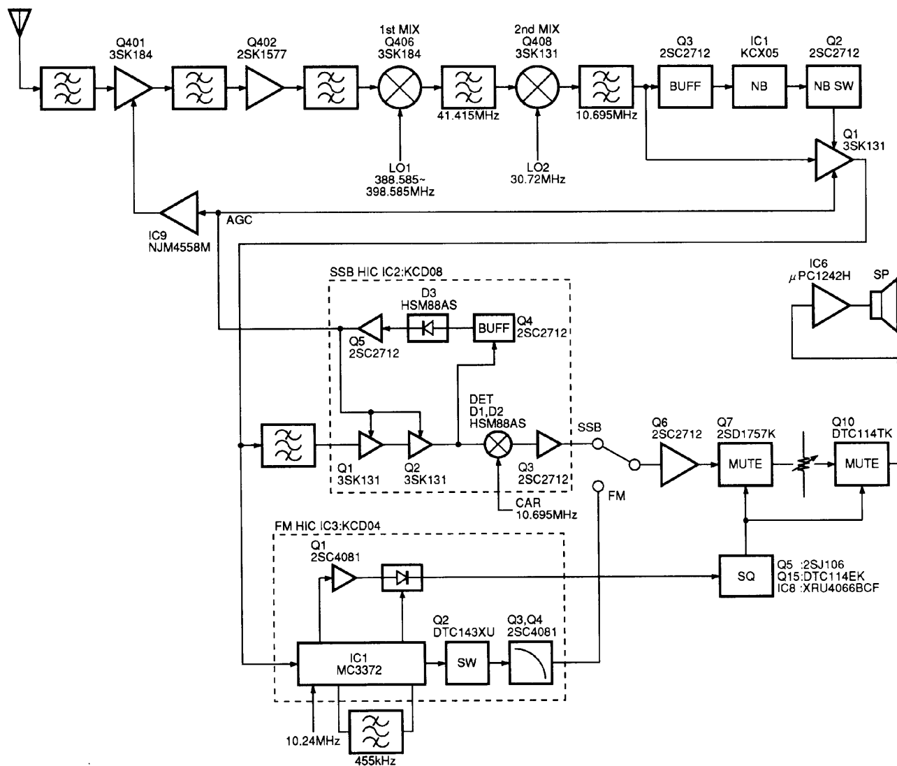
Fig. 4 Receiver circuit block diagram
