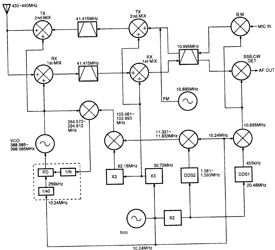
Fig. 2 Transceiver frequency configuration
