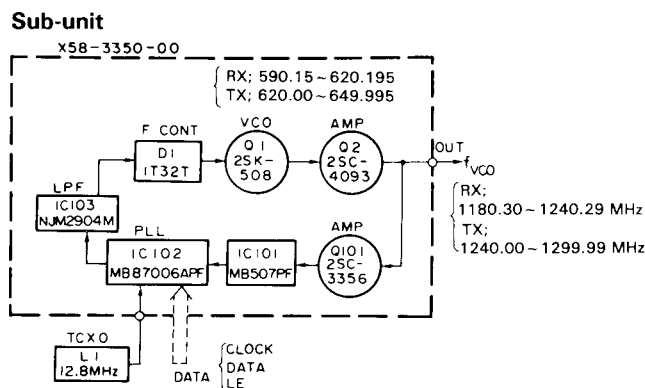
Fig. 6 Block diagram of the PLL unit
