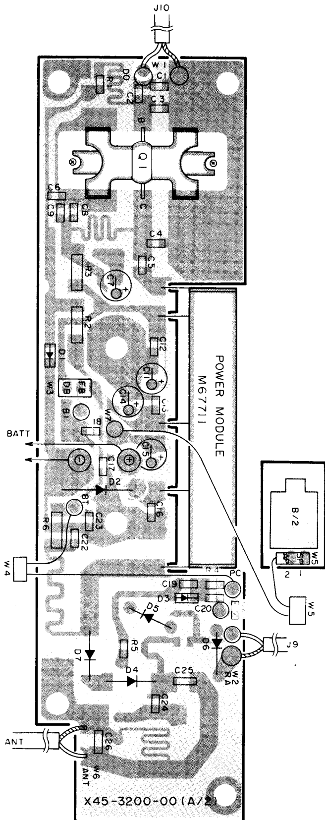
▼ FINAL UNIT (X45-3200-00) (Component side view)
