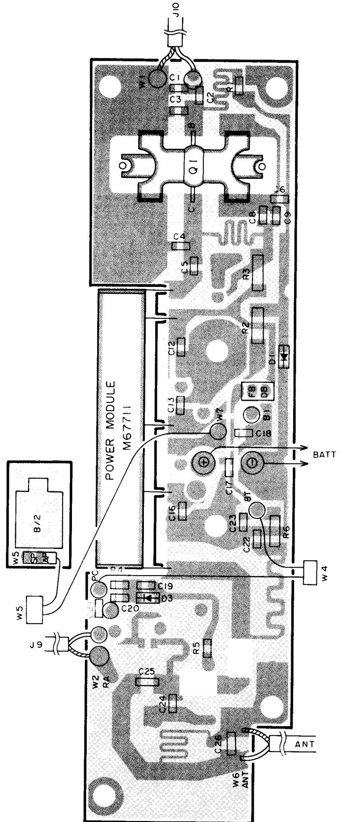
▼ FINAL UNIT (X45-3200-00) (Foil side view)
