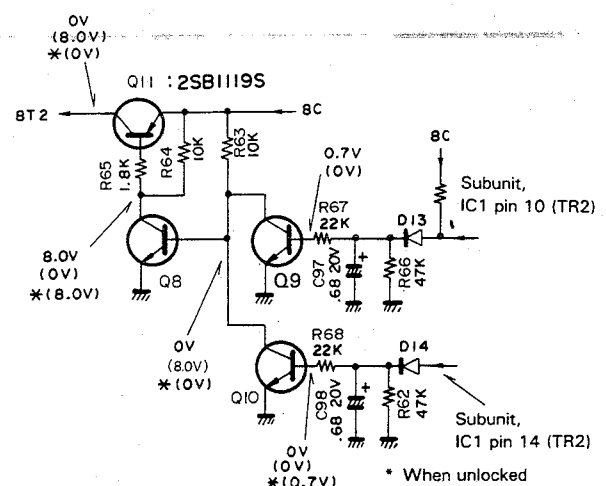
Fig. 11 8T2 (Transmit 8 V) and Transmit Unlock Circuits
