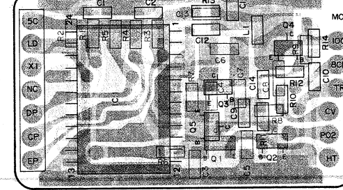
▼144 MHz PLL UNIT A (X58-3670-10) [Foil side view]
