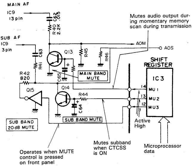
Fig. 8 Mute Circuit
