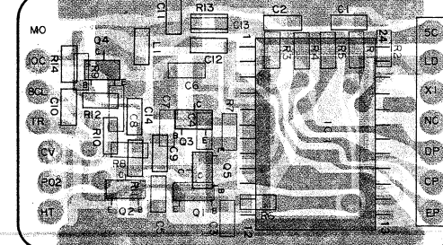
▼144 MHz PLL UNIT A (X58-3670-10) [Component side view]
