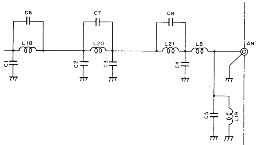
Fig. 7 LPF Circuit
