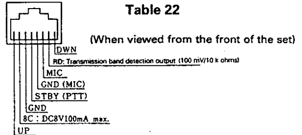
Fig. 43 Microphone Socket (on Front Panel)
