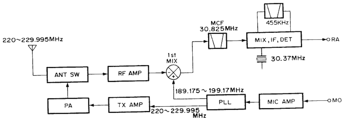
Fig. 14 Frequency configuration
