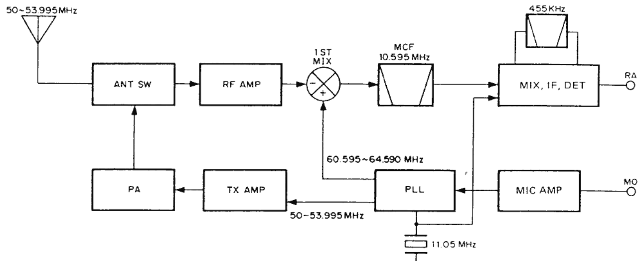
Fig. 5 Frequency Configuration
