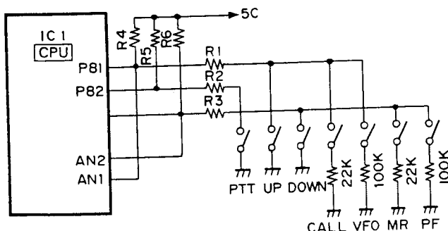
Fig. 37 Microphone key input circuit
