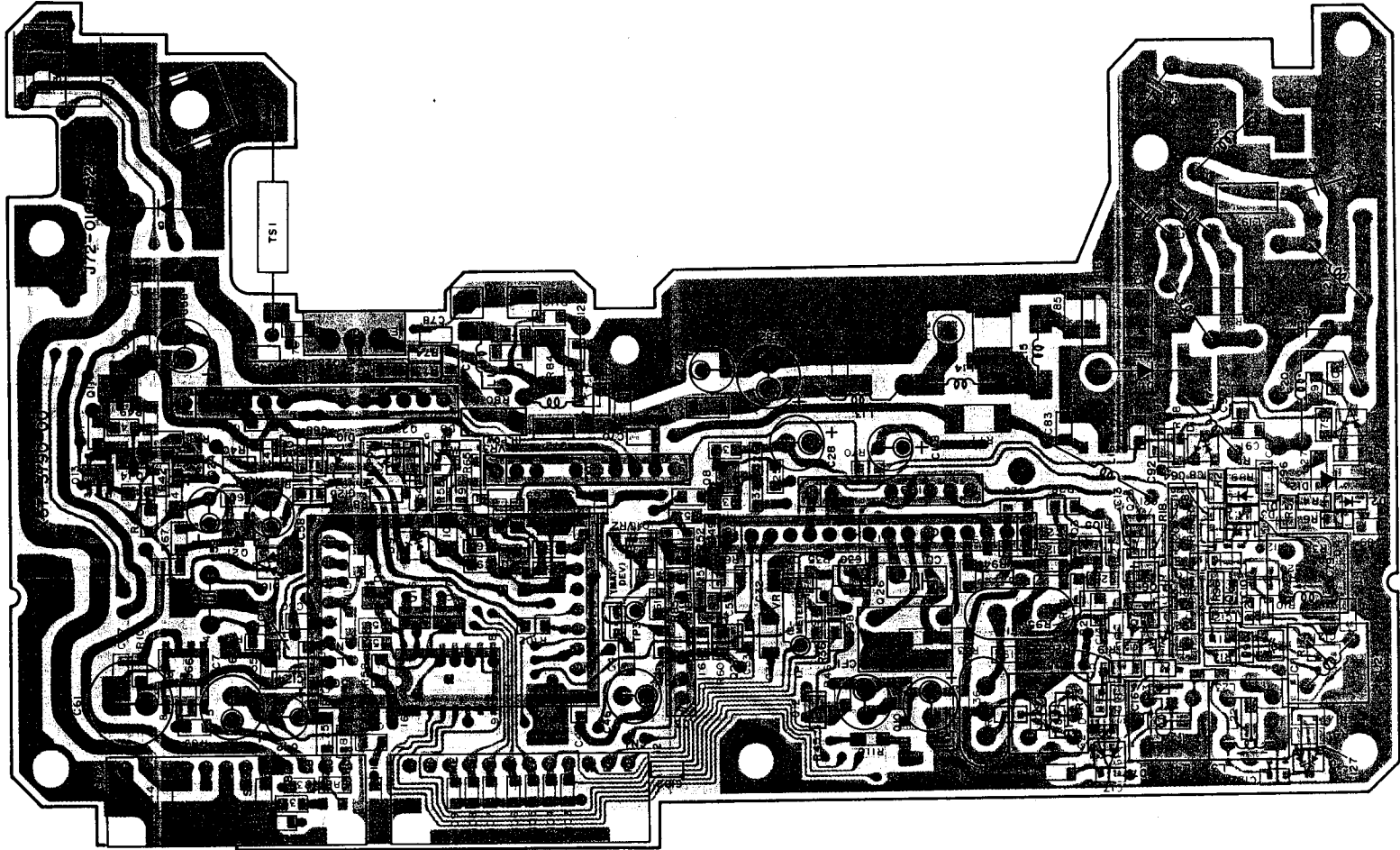
28M TX-RX UNIT (X57-3790-01) Component side view
