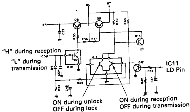
Fig. 23 Unlock Circuit
