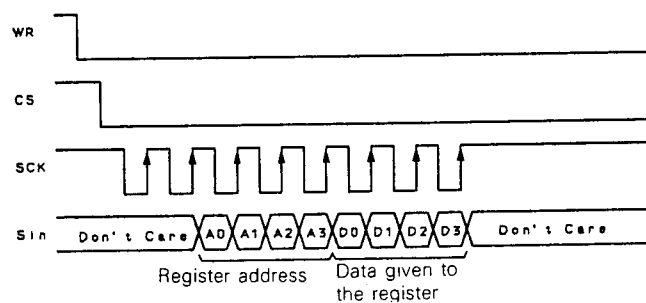
Fig. 31 Register write timing
