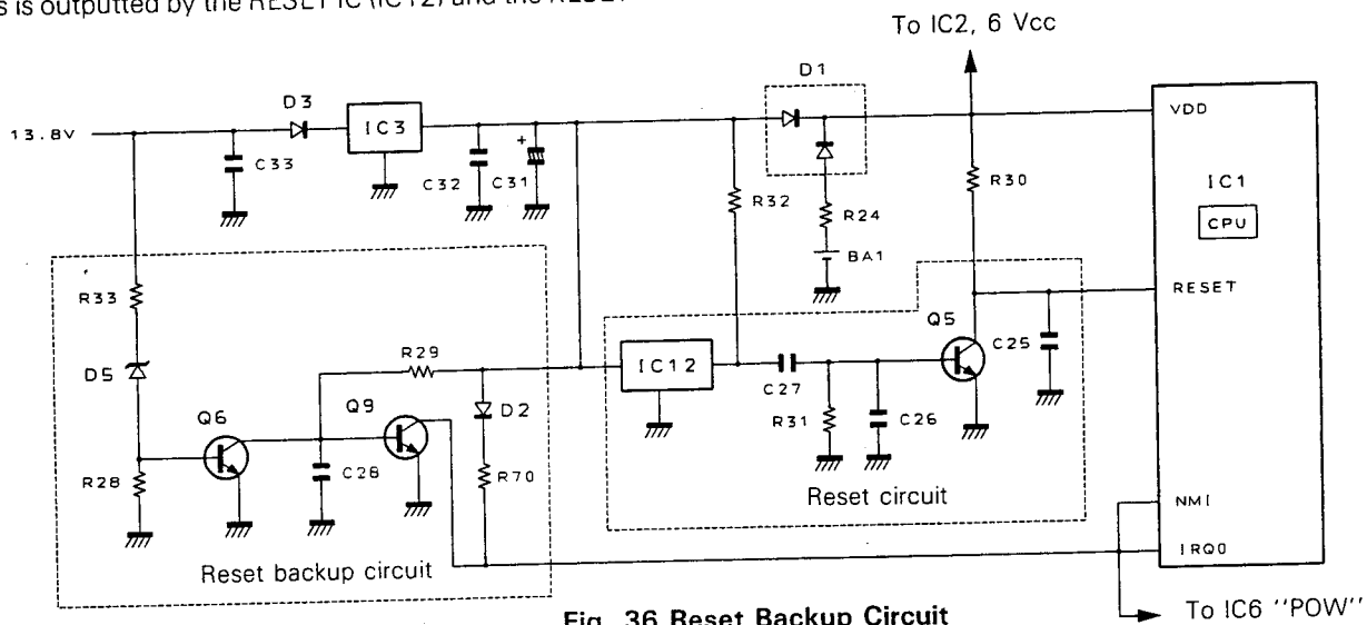
Fig. 36 Reset Backup Circuit
