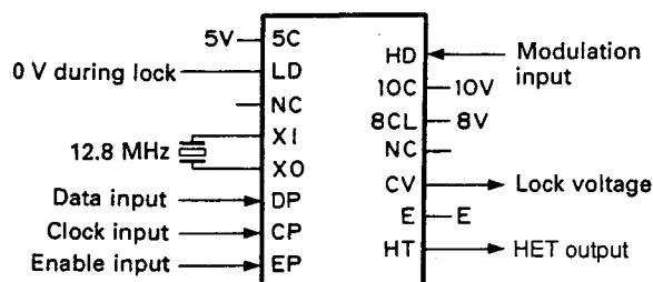
Fig. 12 IC11 KCH05
