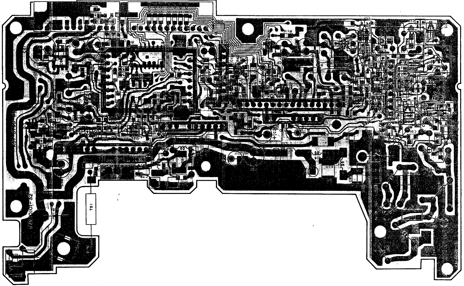
28M TX-RX UNIT (X57-3790-01) Foil side view
