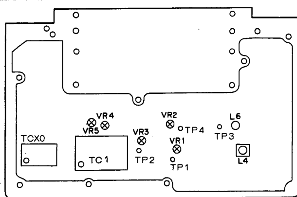
Fig. 59 1200 MHz band adjustment: Component layout (upper view)
