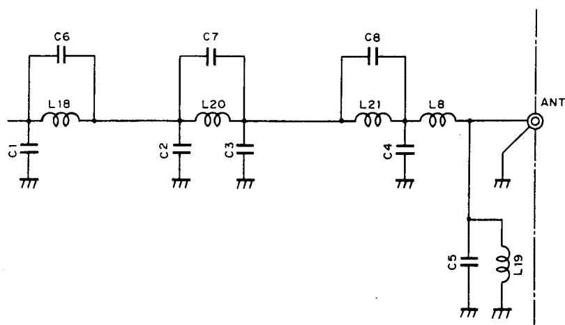
Fig. 7 LPF Circuit
