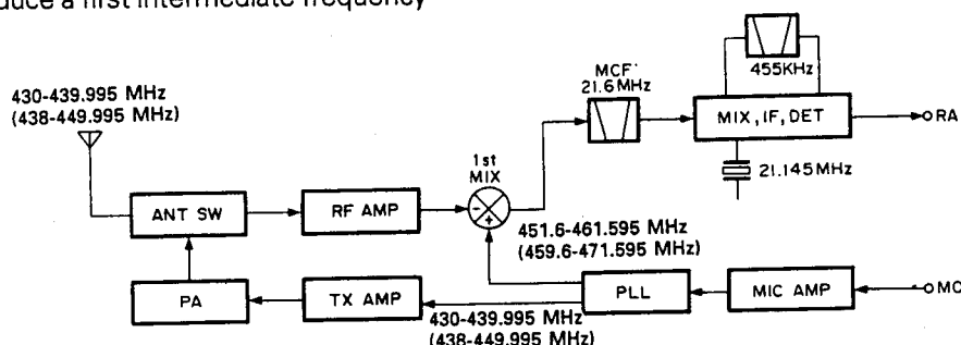
Fig. 16 Frequency Configuration
