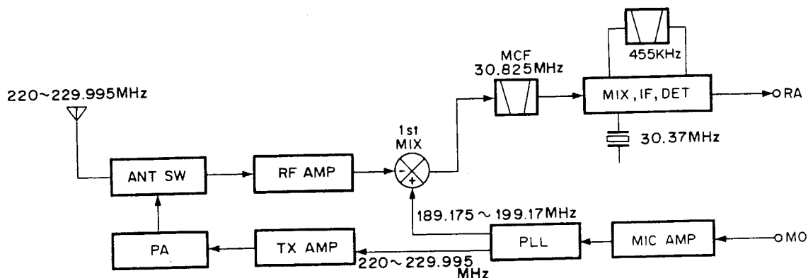
Fig. 14 Frequency configuration
