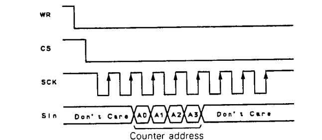
Fig. 30 Counter write timing
