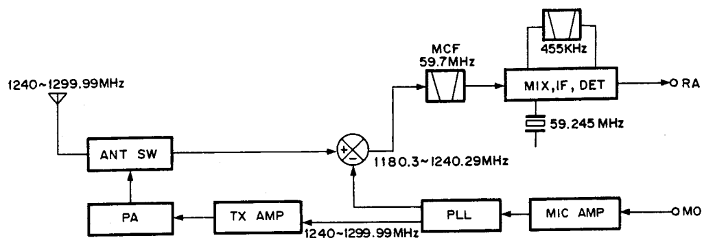
Fig. 18 Frequency Configuration
