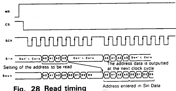
Fig. 28 Read timing
