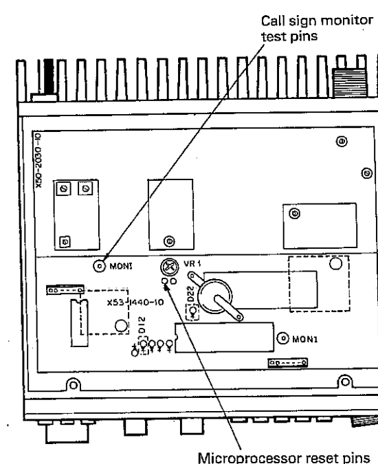
Bottom view
