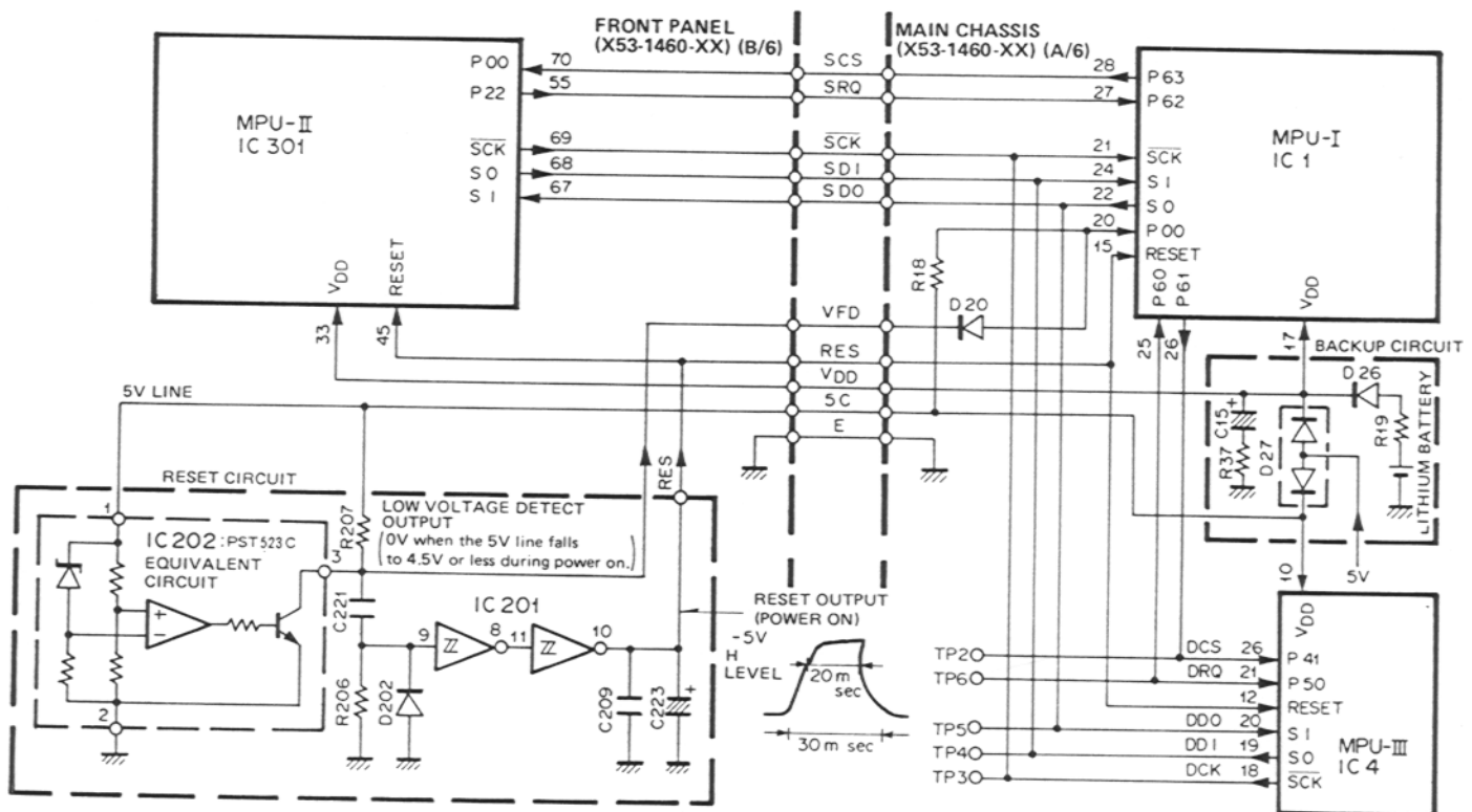
Fig. 9 Interface between MPUs and reset backup circuit
