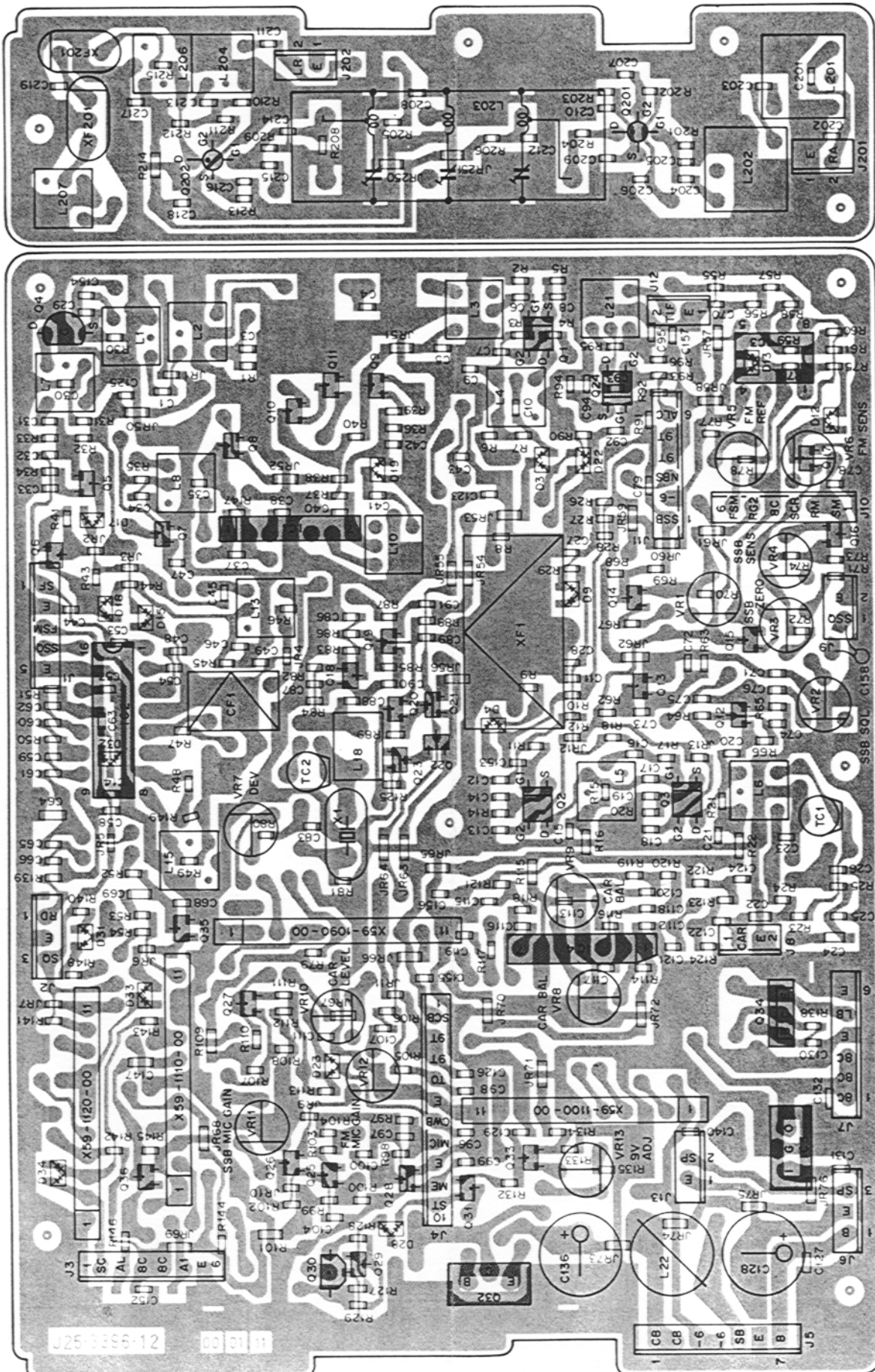
COMPOSITE UNIT (RX) (X60-1320-00) S/N. 705-707XXXX : W,T Foil side view
