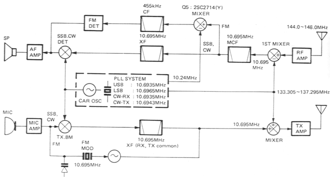
Fig. 1 Frequency configuration
