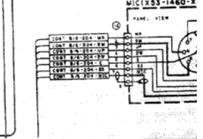
CONTROL UNIT (X53-1460-XX)
