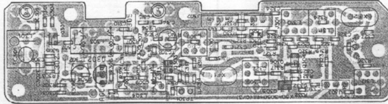
COMPOSITE UNIT (PLL,DRIVE,FRONT)(X50-3050-11) Component side view
