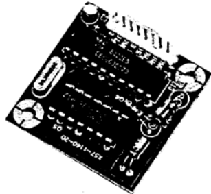
MU-1 PC BOARD VIEW (X57-1140-20) Component side view
