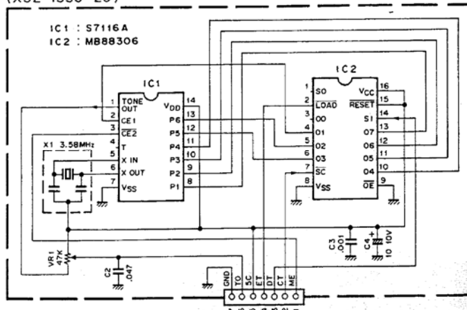
TU-7 SCHEMATIC DIAGRAM
