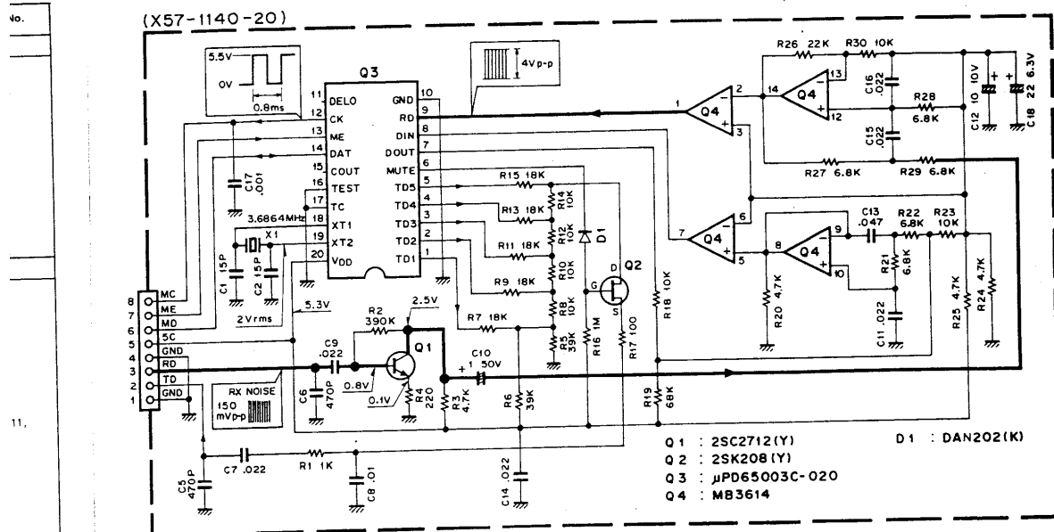
MU-1 SCHEMATIC DIAGRAM
