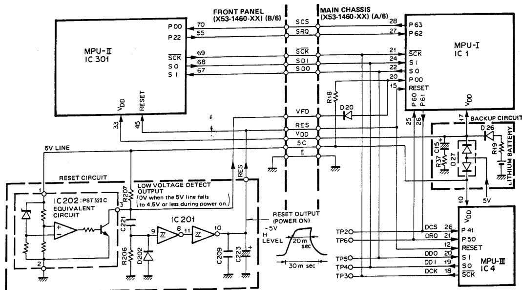
Fig. 9 Interface between MPUs and reset backup circuit
