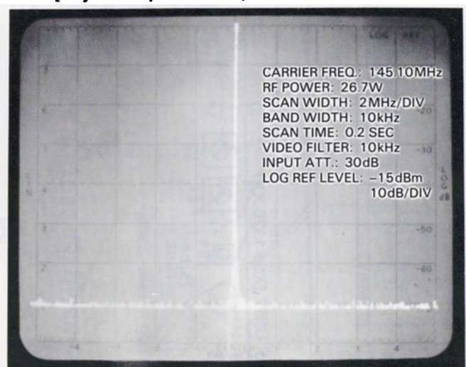
[Adjacent spurious response characteristic]
