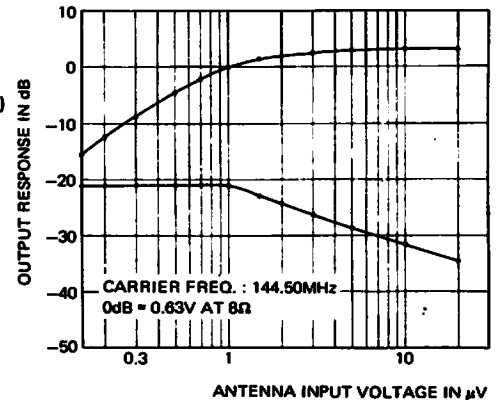
[Reception sensitivity characteristics] USB mode
