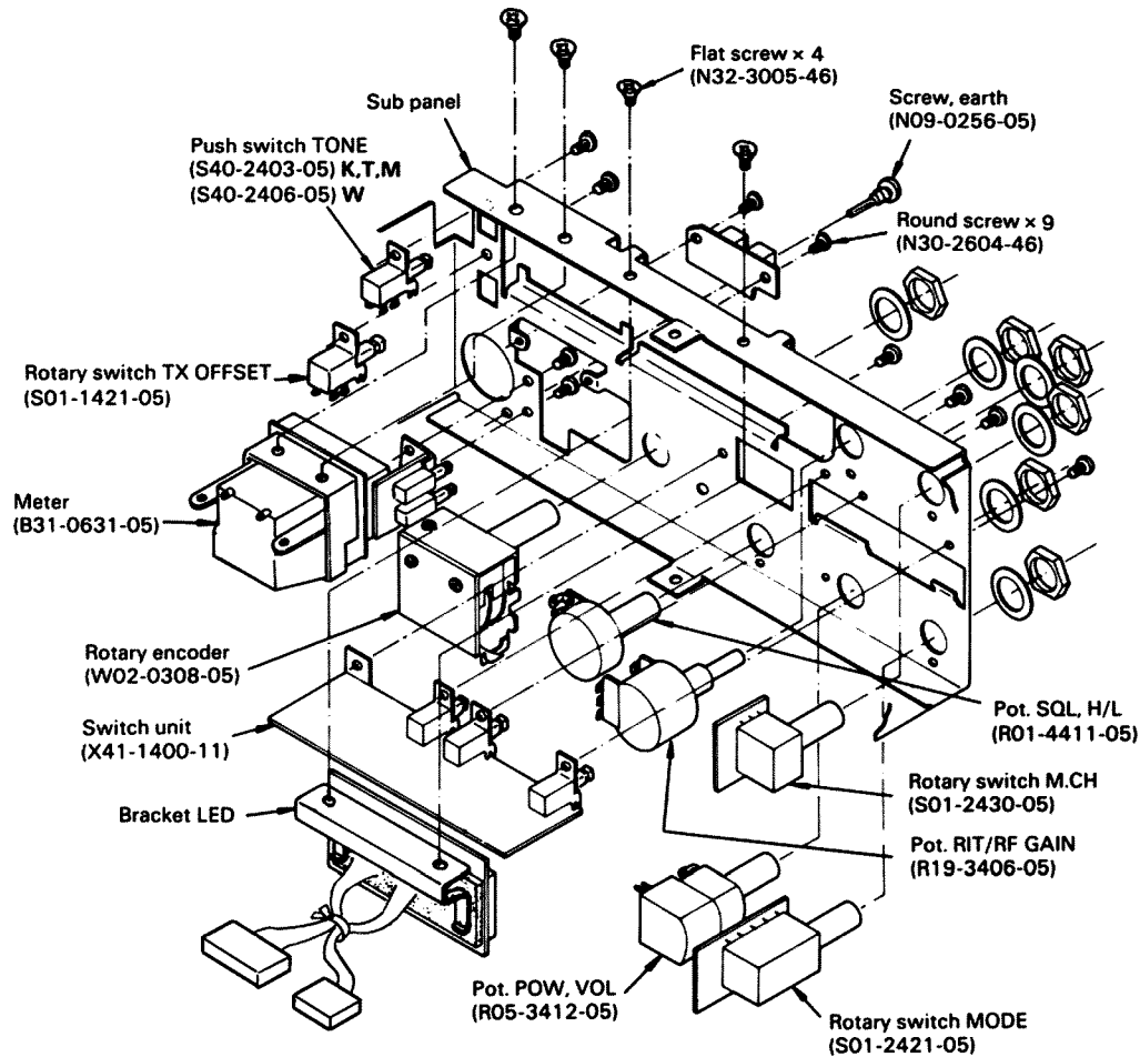
Fig. 21 Sub panel
