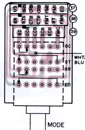
MODE UNIT (J25-3099-04) [Component Side View]
