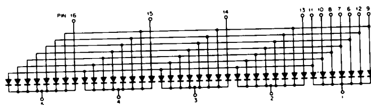
Fig. 9 5 digit LED SL-2504K
