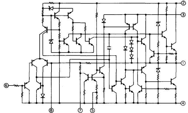
Fig. 1 MB3713 Equivalent circuit (RX unit Q38)
