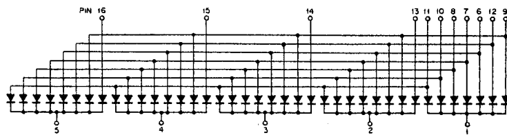
Fig. 6 5 digit LED SL-2504K
