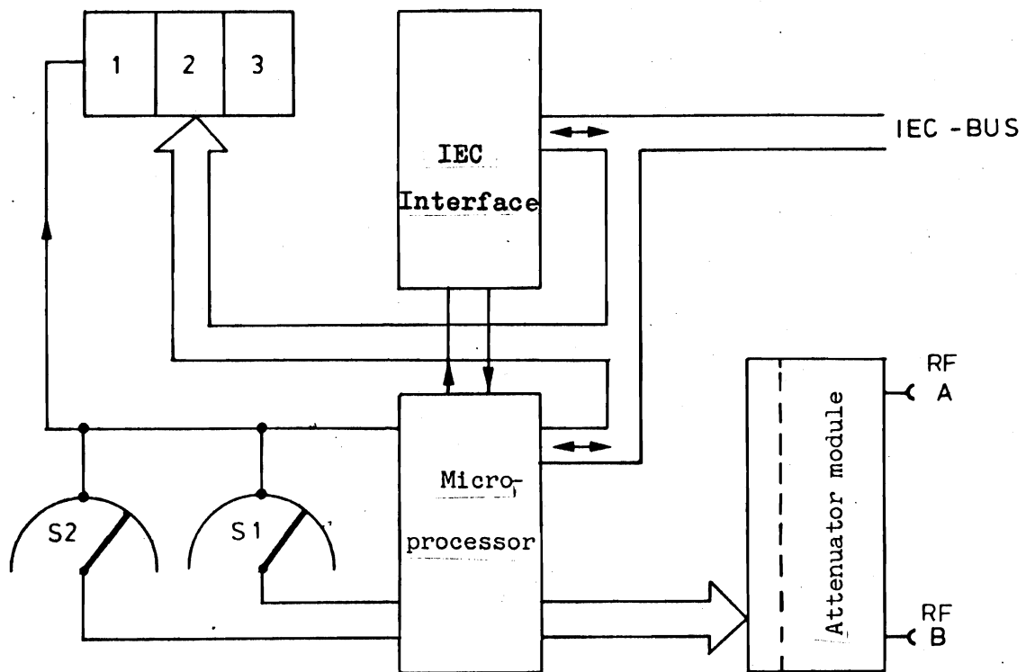
Fig. 4 Block diagram
