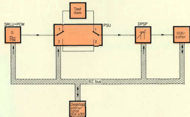
Automatic test assembly for attenuation and gain measurements using programmable RF Step Attenuator DPSP
