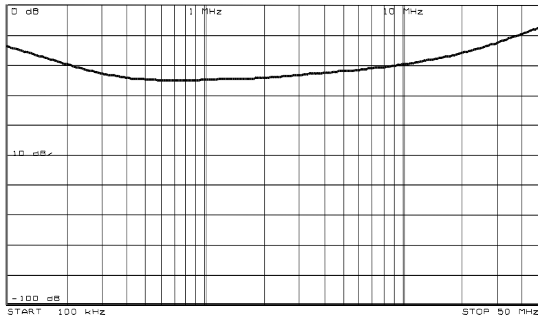
Fig. 5 Attenuation of sheath current choke measured in 150 \Omega test setup
