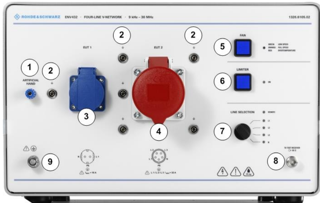
Fig. 1 Front View
