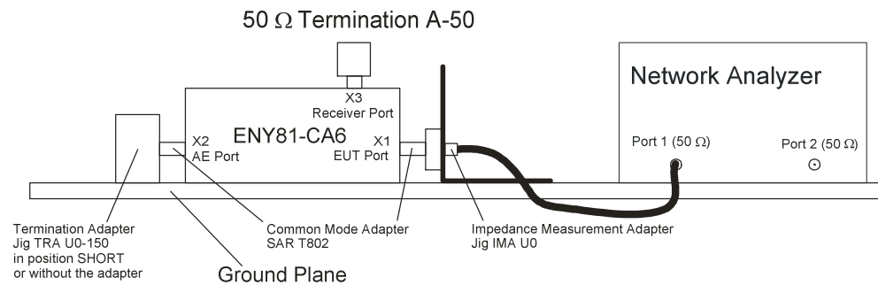
Fig. 6 Test set-up for Asymmetrical Impedance and Phase in accordance with CISPR 16-1-2 for R&S ENY81-CA6
