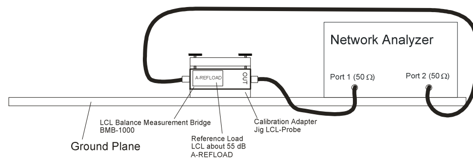
Fig. 15 Validation of the LCL balance measurement bridge
