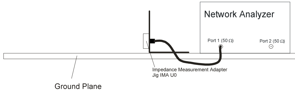
Fig. 2 Calibration set-up "Open" for Asymmetrical Impedance and Phase
