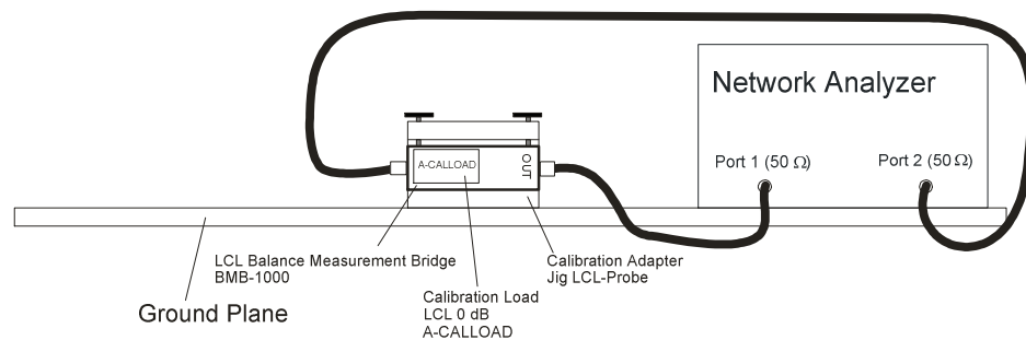
Fig. 14 Normalization of the LCL balance measurement bridge
