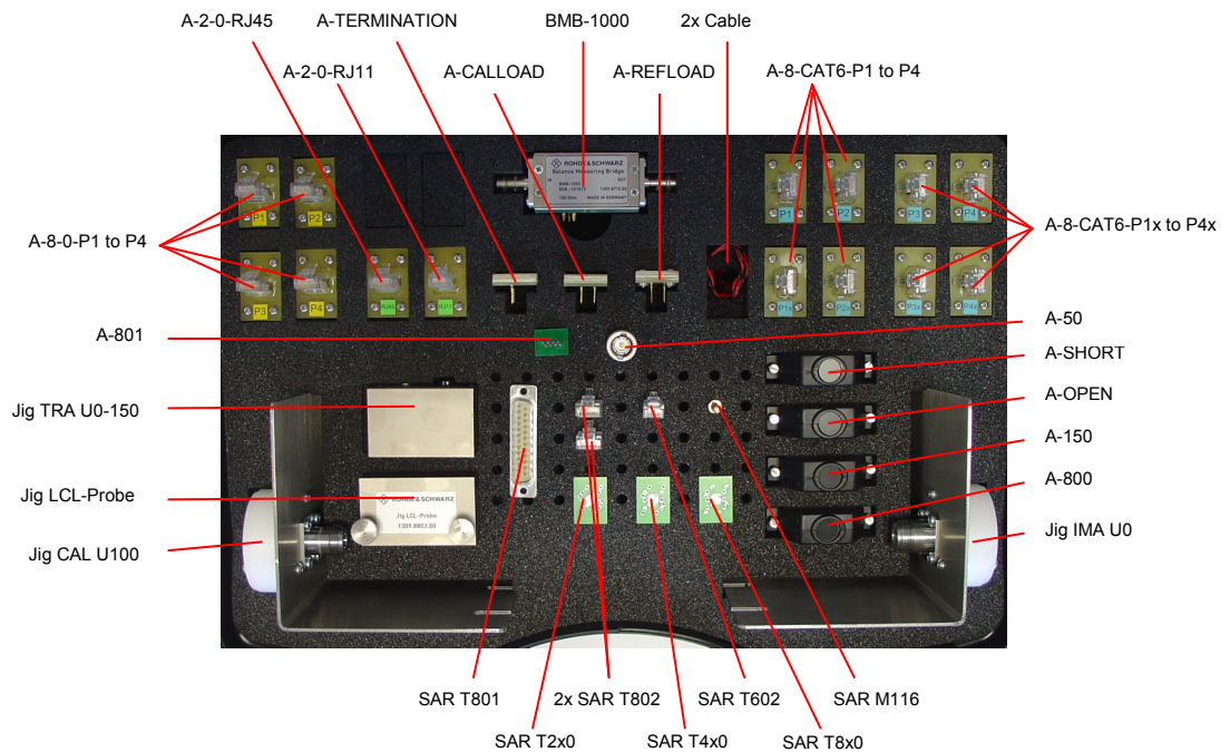
Fig. 1 Parts of the R&S ENY-FTS
