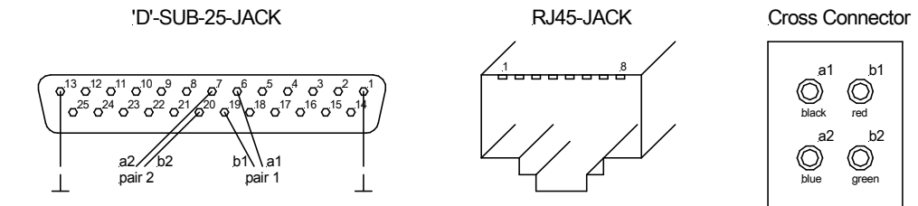
Fig. 3 Connector assignments
