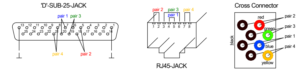
Fig. 3 Connector assignments
