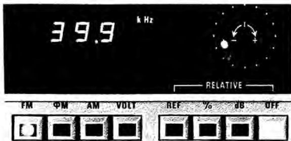
Front-panel section: middle display/keyboard for modulation measurement results and operating mode selection
