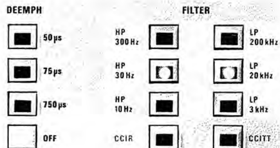
Front-panel section: middle keyboard for weighting bandwidths and FM deemphasis
