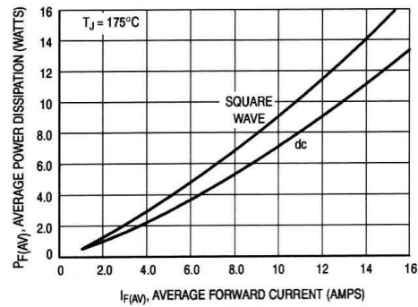
Figure 5. Power Dissipation (Per Leg)
