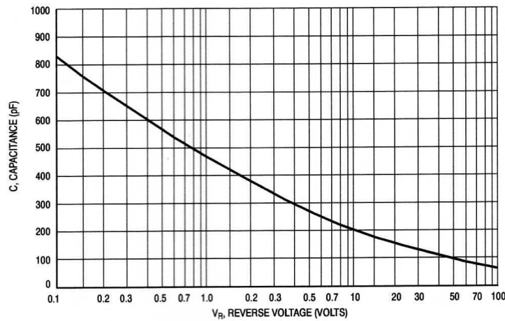
Figure 7. Typical Capacitance (Per Leg)
