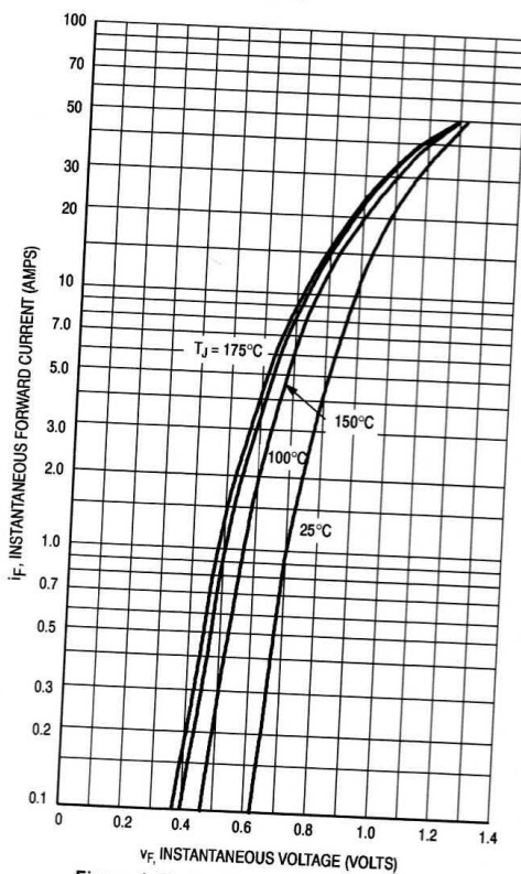
Figure 1. Typical Forward Voltage (Per Leg)
