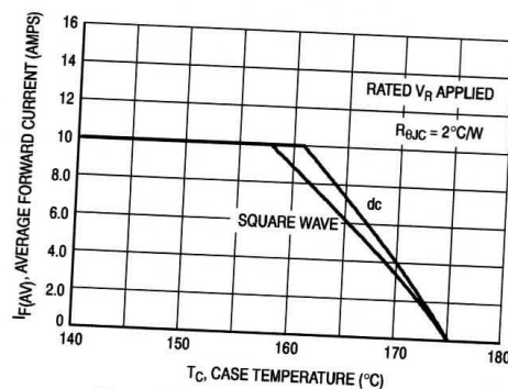
Figure 3. Current Derating, Case (Per Leg)
