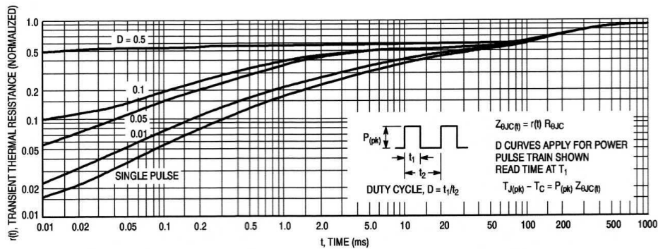
Figure 6. Thermal Response
