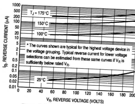
Figure 2. Typical Reverse Current* (Per Leg)
