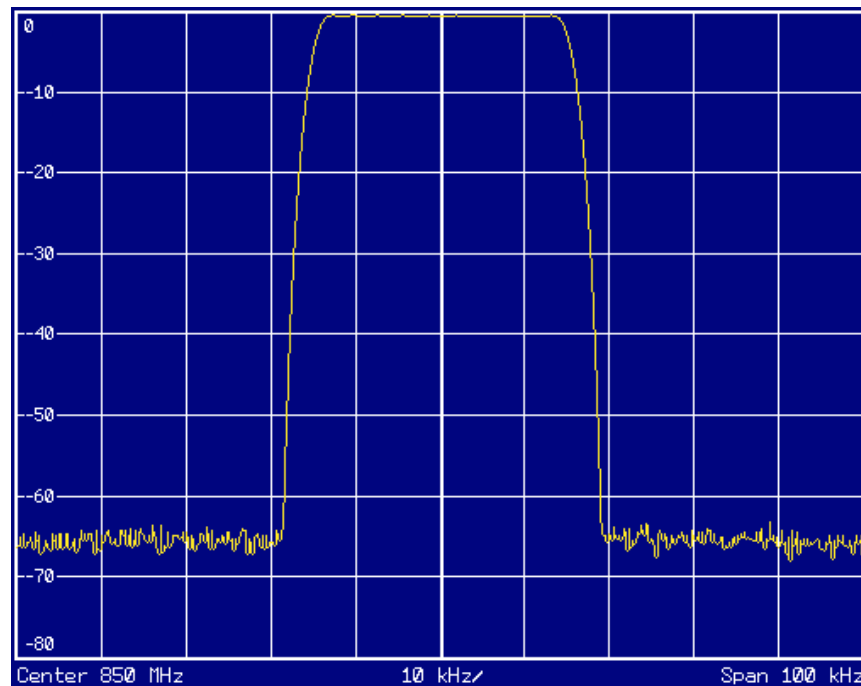
Fig. 2.26 Frequency response of the 30 kHz channel filter for measuring the power in the IS 95 adjacent channel
