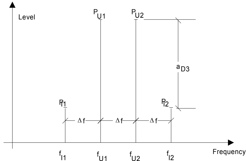
Fig. 4.14 Intermodulation products P_{U1} and P_{U2}
