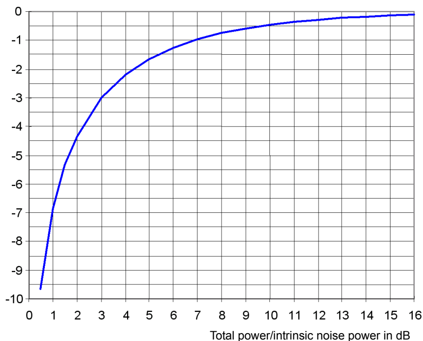
Fig. 2.13 Correction factor for measured noise power as a function of the ratio of total power to the intrinsic noise power of the R&S FSG.
