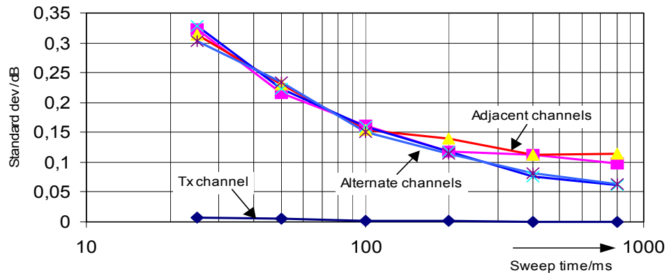
Fig. 2.25 Repeatability of adjacent channel power measurements on IS95 signals in the Fast ACP mode
