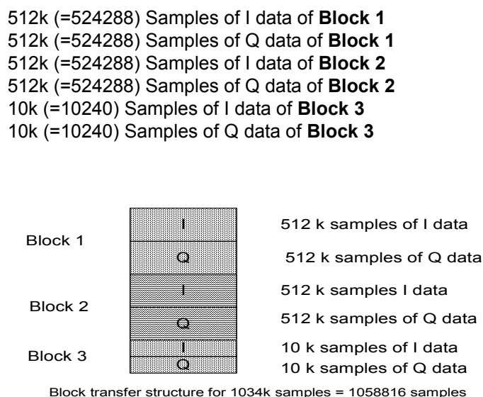
Fig. 6.2 Block transfer structure
