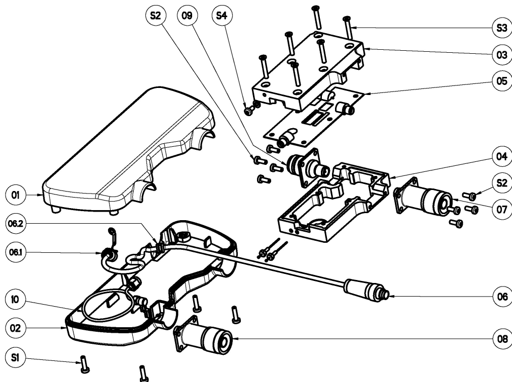
Fig. 3-4 Exploded View
