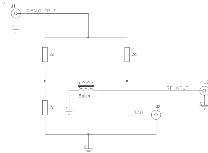
Fig. 3-2 Principle Diagram: Circuit in SWR Bridge state
