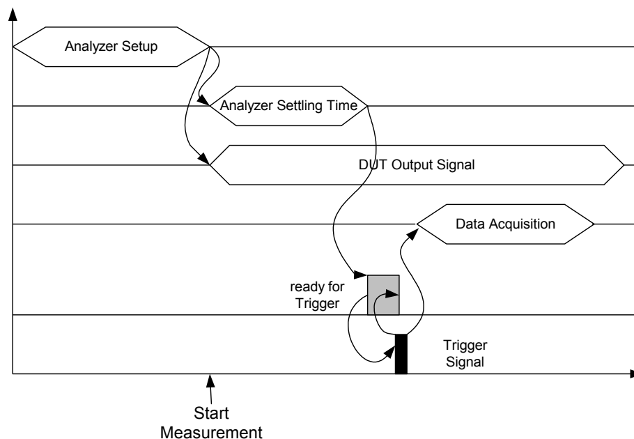
Fig. 4.45 Test with ready-for-trigger signal
