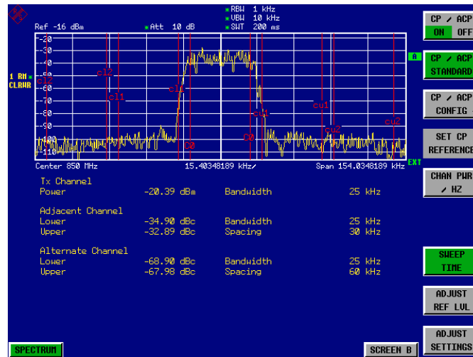
Fig. 2-1 Measuring the relative adjacent channel power of an NADC signal in each of the two adjacent channels below and above the transmit channel.
