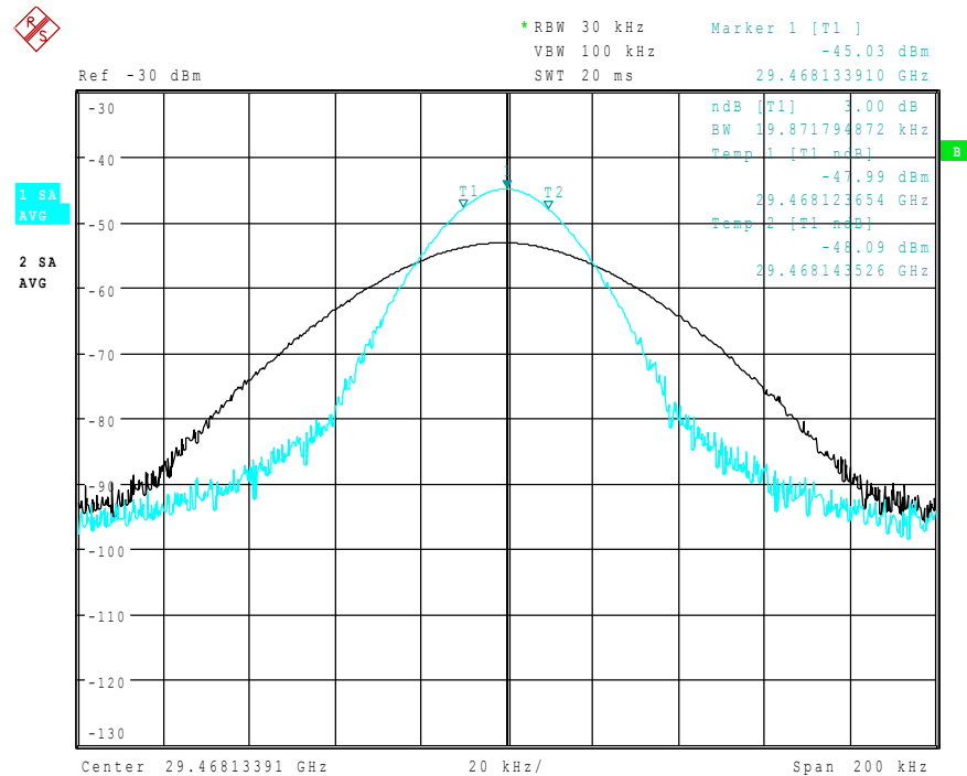
Fig. 4.39 Different mixer products represented at the same frequency in the test sweep and reference sweep
