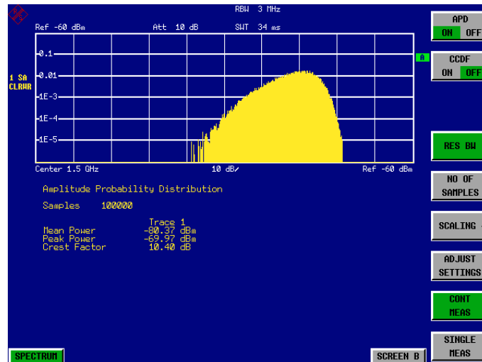
Fig. 2-1 Amplitude probability distribution of white noise
