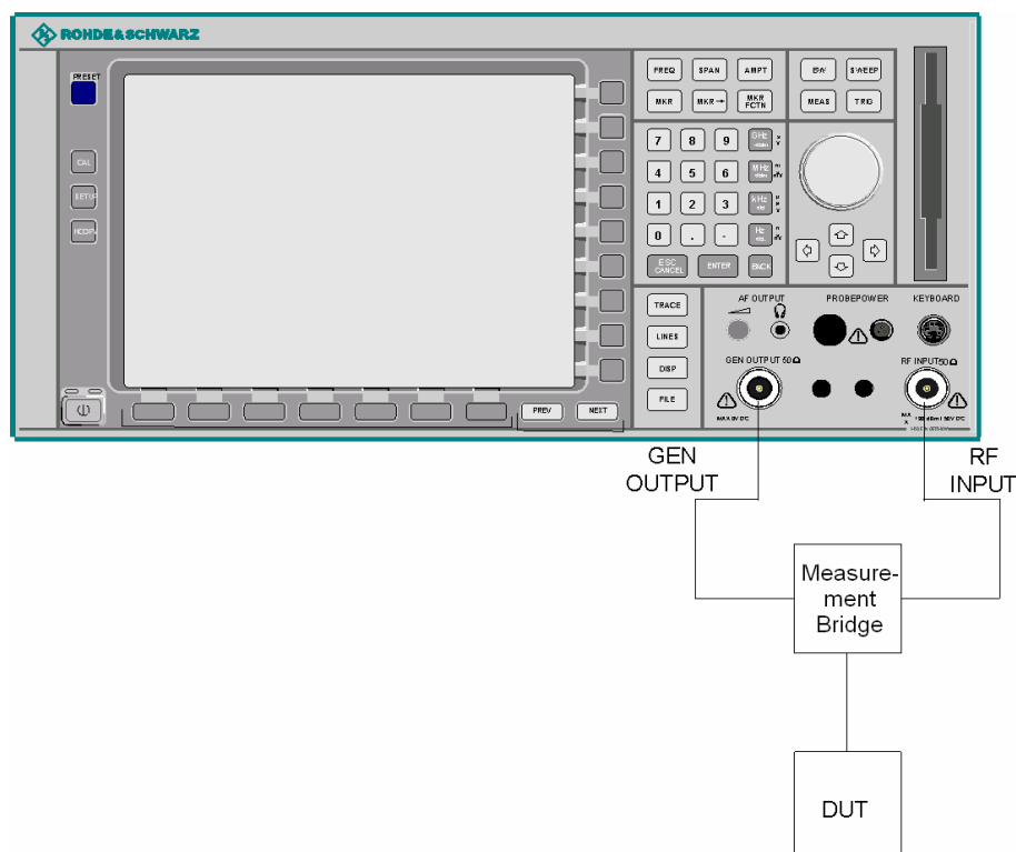
Fig. 4.25 Test Setup for Reflection Measurement
