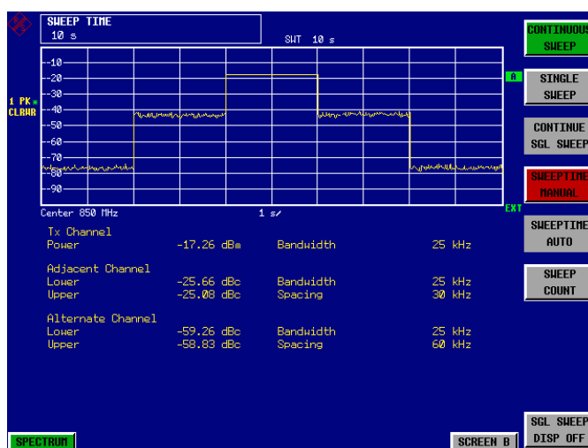
Fig. 2-5 Adjacent channel power due to modulation spectrum and transient spectrum
