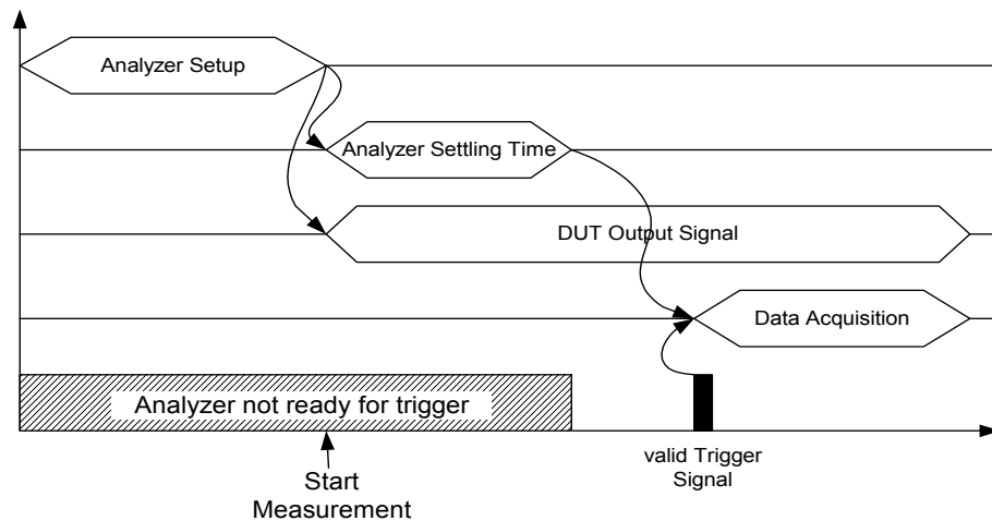
Fig. 4.44 Test with single trigger pulse
