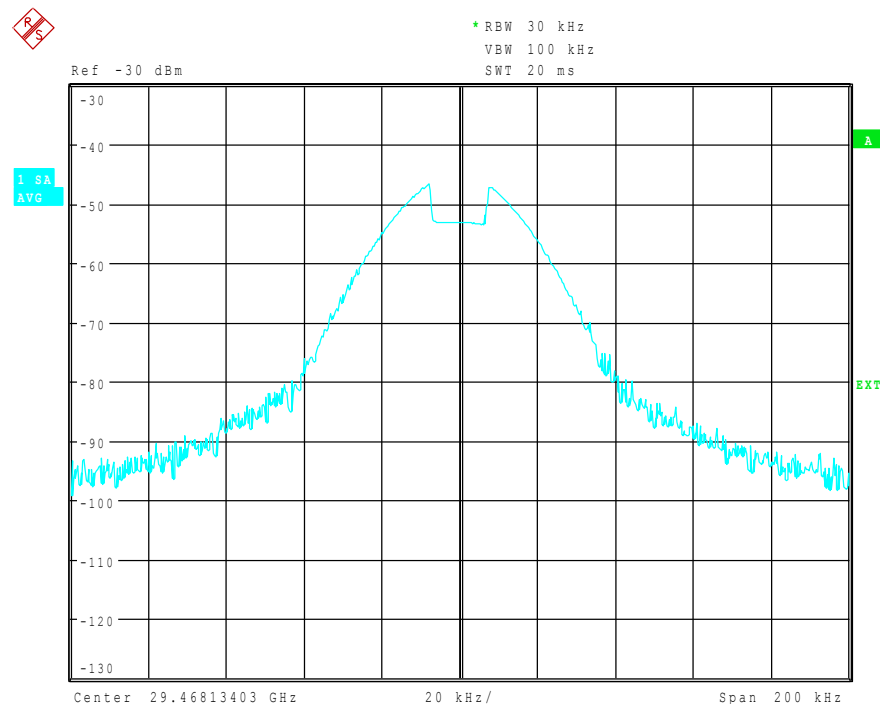
Fig. 4.40 Signal as in Fig. 4.38, but with the use of AUTO ID
