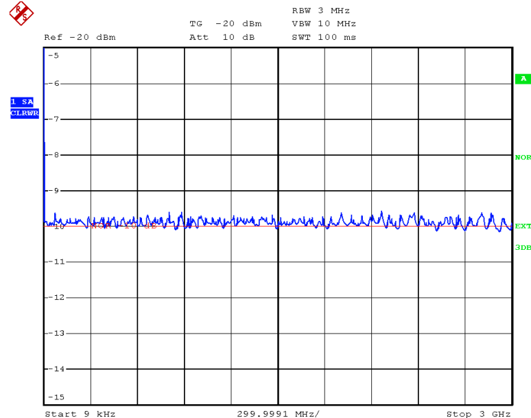
Fig. 4.24 Measurement of a 10dB attenuator pad with 1dB/DIV
