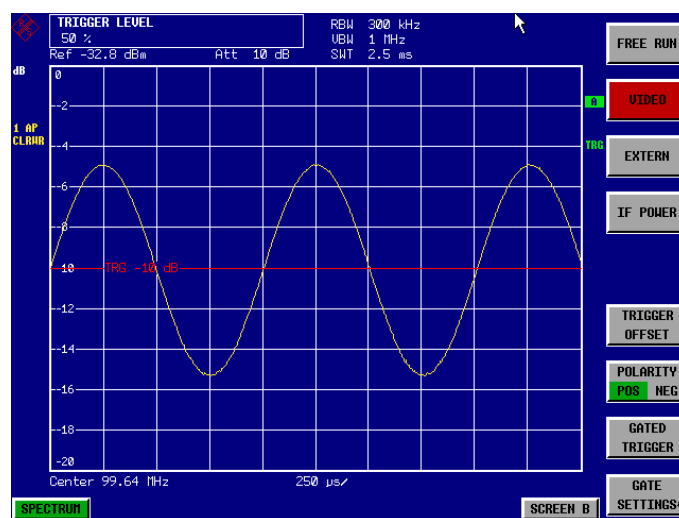
Fig. 2.18 Demodulated FM signal
