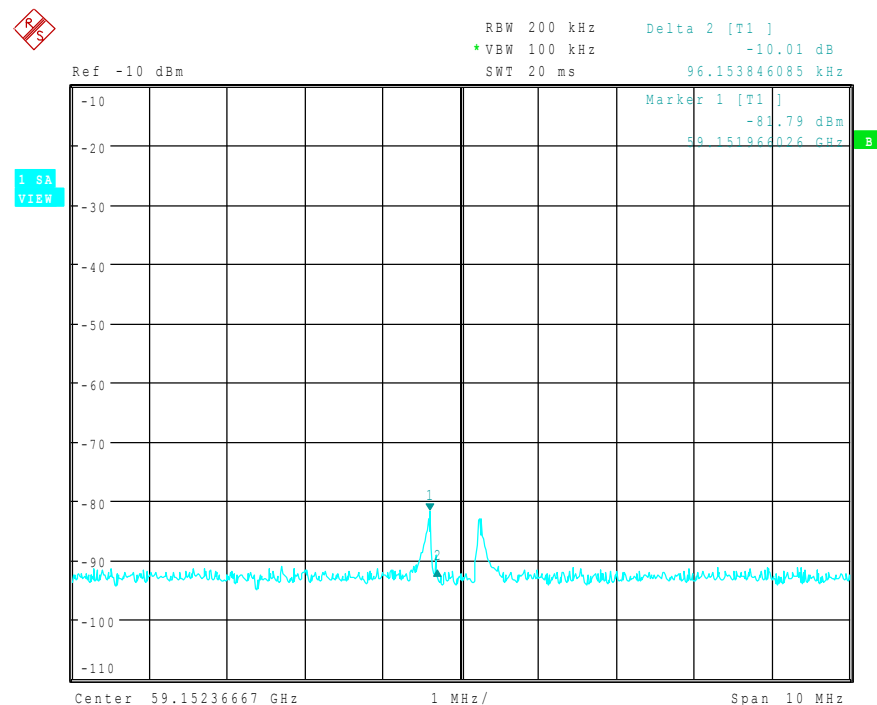
Fig. 4.37 Components of a mixer product blanked out with AUTO ID
