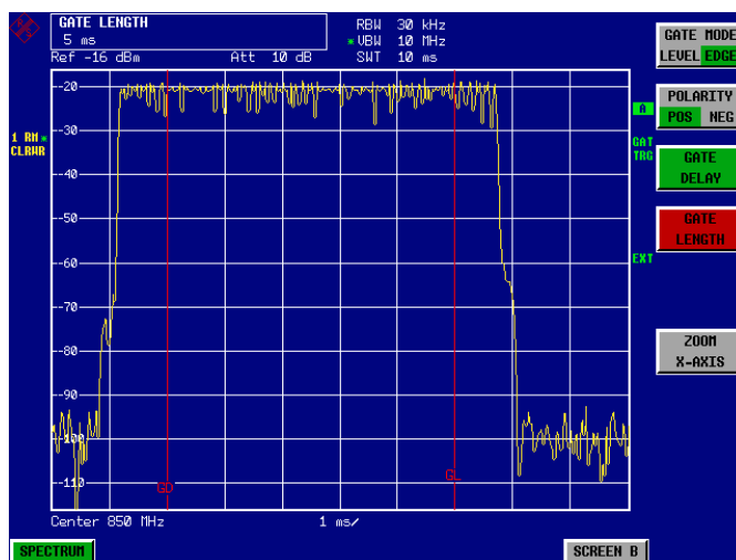
Fig. 2-4 Setting the parameters Gate Delay and Gate Length in time domain. The time interval required to measure the spectrum is indicated by two vertical lines.
