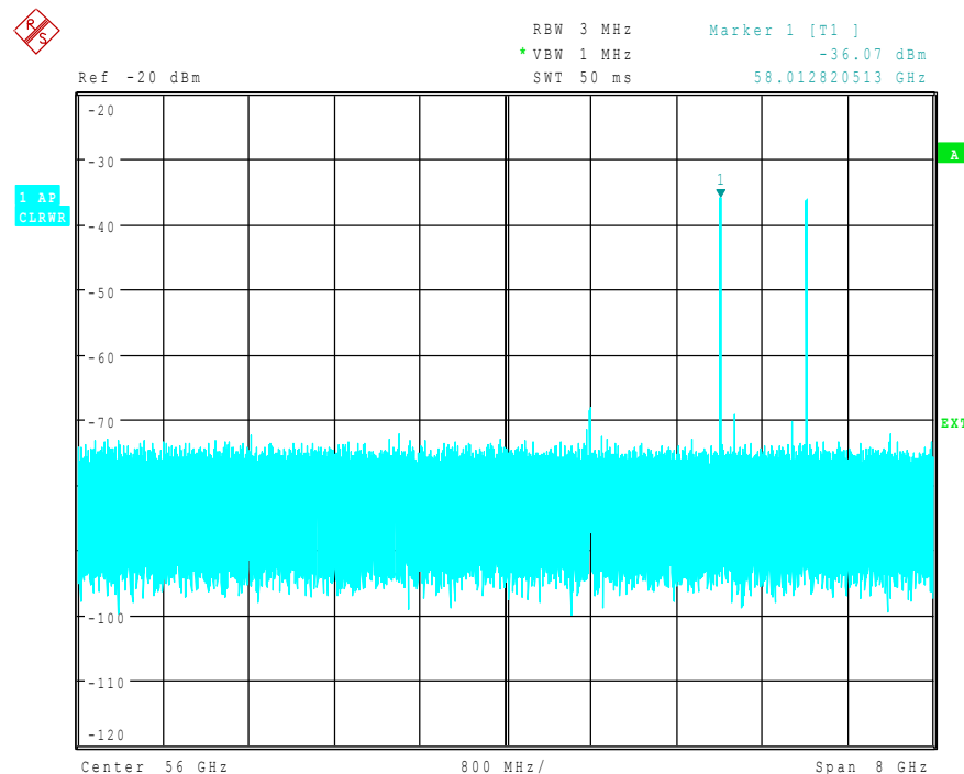
Fig. 4.41 Spectrum at the multiplier output recorded with an external mixer
