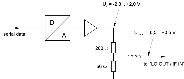
Fig. 4.36 Bias circuit of the R&S FSP
