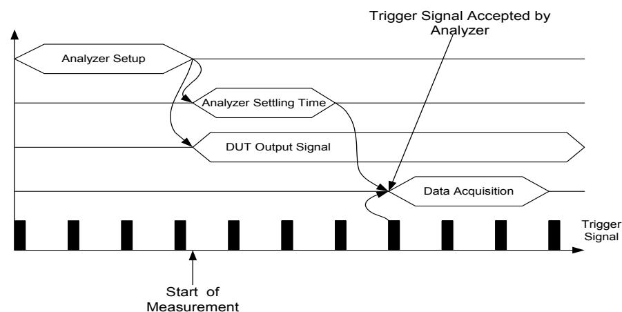
Fig. 4.43 Test with stationary test signal and periodic trigger signal
