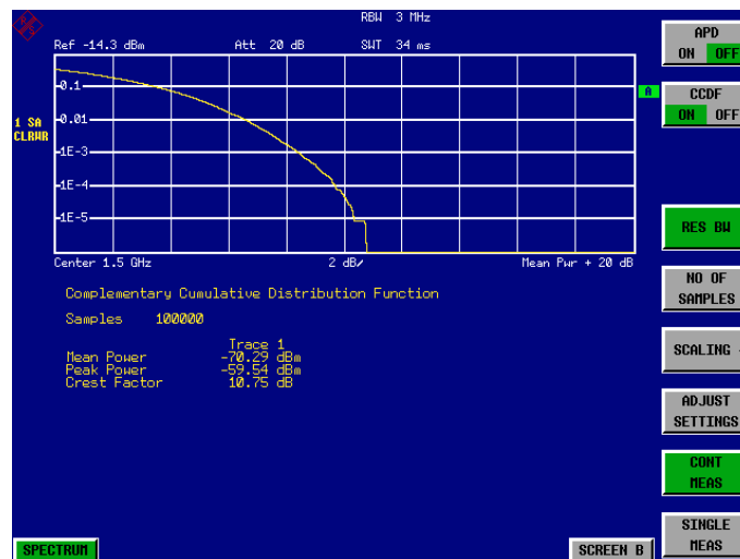
Fig. 2-2 The CCDF of white noise
