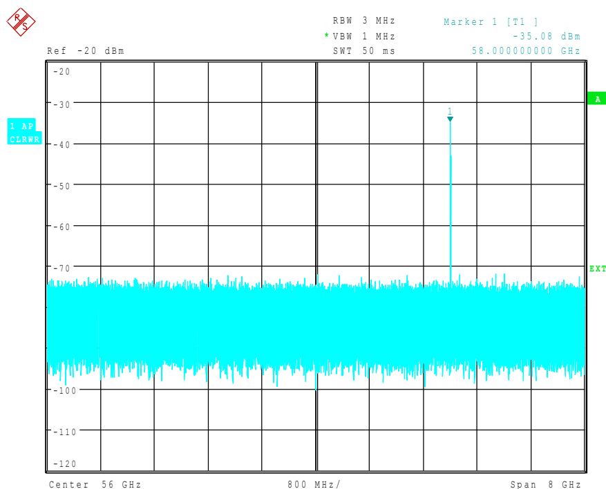
Fig. 4.42 Output spectrum of the multiplier recorded with an external mixer and AUTO ID
