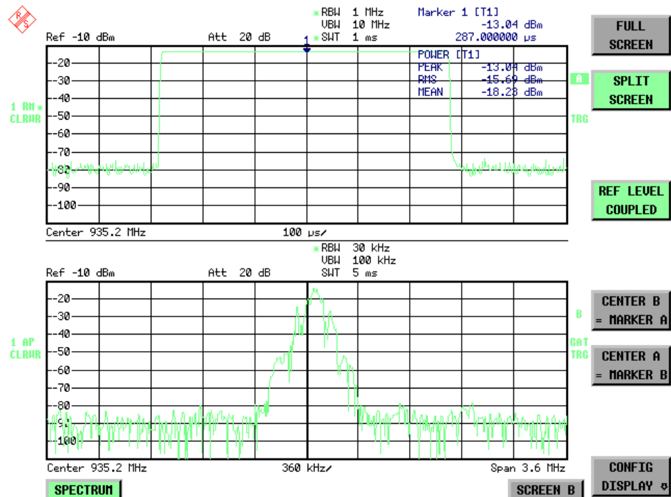
Fig. 4.16 Typical split-screen display, settings are uncoupled
