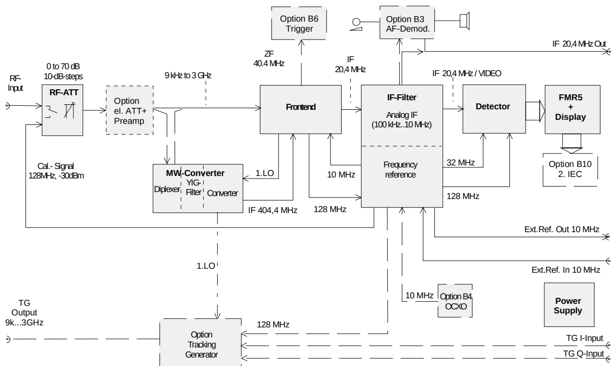
Fig. 3-1 Block diagram
