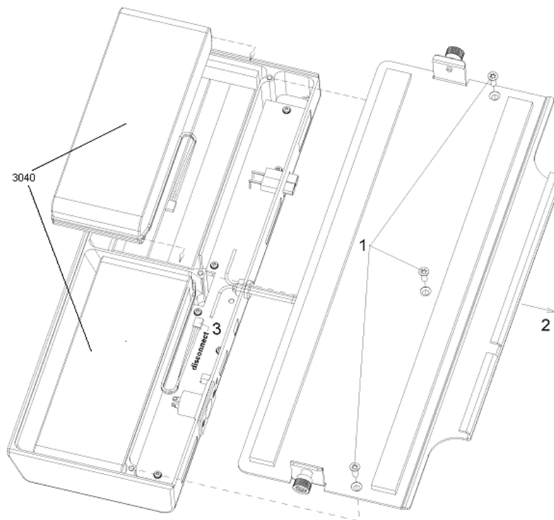
Fig. 3-3 Removing and installing the batteries, FSP-B31/B32
