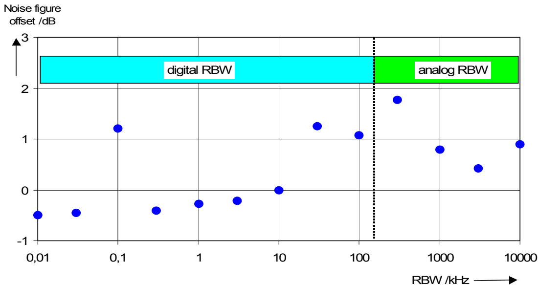
Fig. 2-8 Change in R&S FSU noise figure at various bandwidths. The reference bandwidth is 10 kHz
