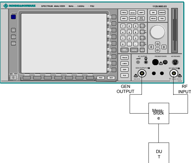
Fig. 4-24 Test Setup for Reflection Measurement
