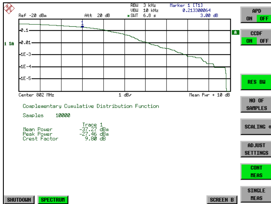
Fig. 4-11 Display of the complementary cumulative distribution function (CCDF)
