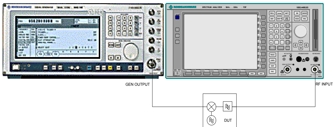
Fig. 4-34 Test setup for frequency-converting measurements
