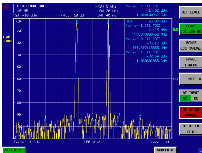
Fig. 2-4 If the RF attenuation is increased, the R&S FSU's intrinsic intermodulation products disappear below the noise floor.
