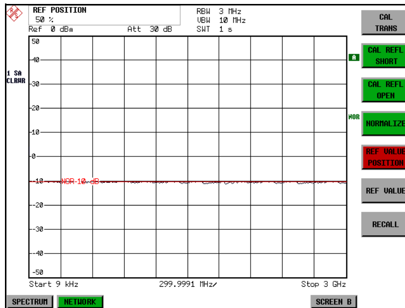
Fig. 4-22 Measurement with REF VALUE -10 dB and REF VALUE POSITION 50%
