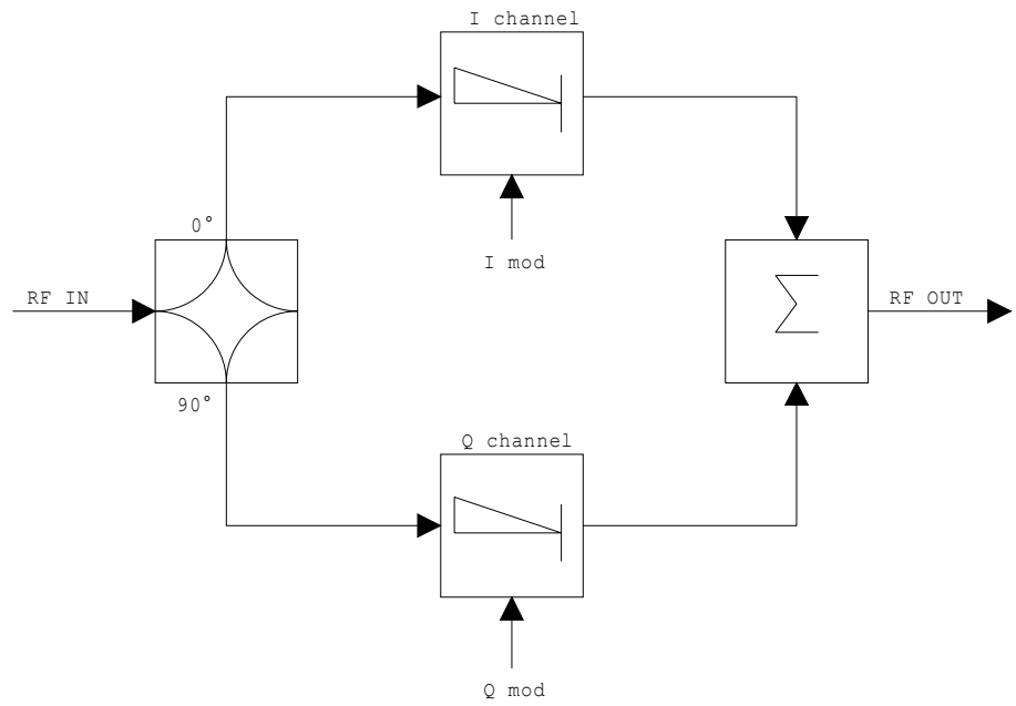
Fig. 4-26 I/Q modulation
