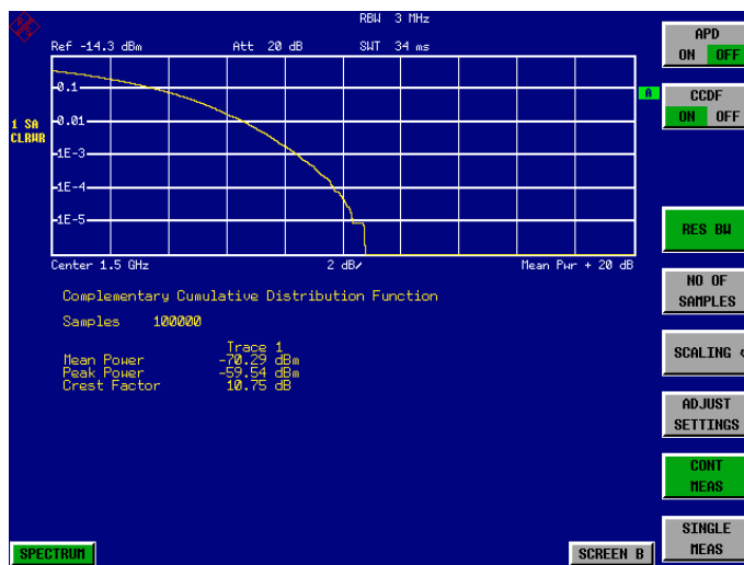
Fig. 2-36 The CCDF of white noise
