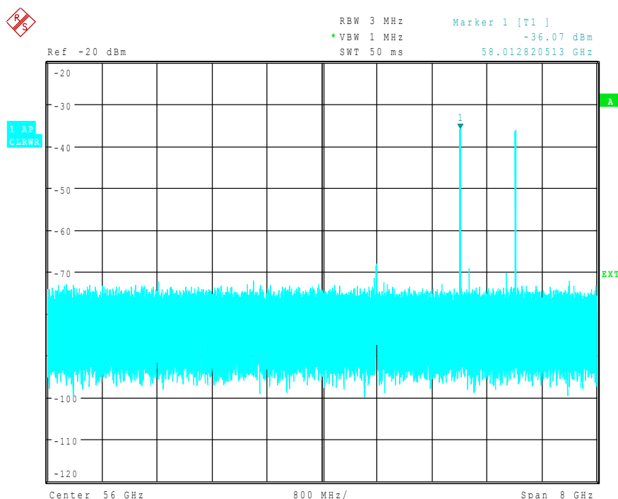
Fig. 4-40 Spectrum at the multiplier output recorded with an external mixer
