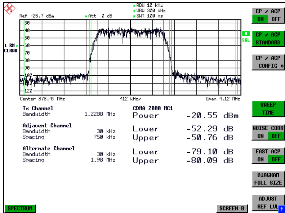
Fig. 4-7 Screen display of adjacent-channel power measurement using the IBW method
