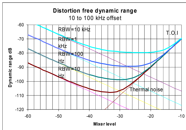
Fig. 2-6 Intermodulation-free dynamic range of the FSU3 as a function of level at the input mixer and of the selected resolution bandwidth (useful signal offset = 10 to 100 kHz, DANL = -157 dBm /Hz, TOI = 25 dBm; typ. values at 2 GHz).
