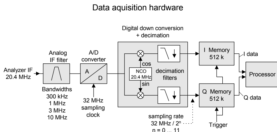
Fig. 6-1 Block diagram illustrating the R&S FSU signal processing
