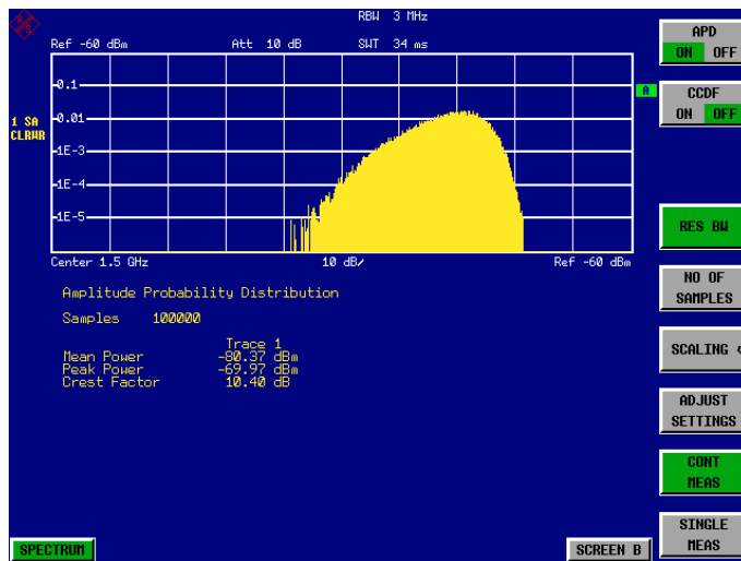
Fig. 2-35 Amplitude probability distribution of white noise
