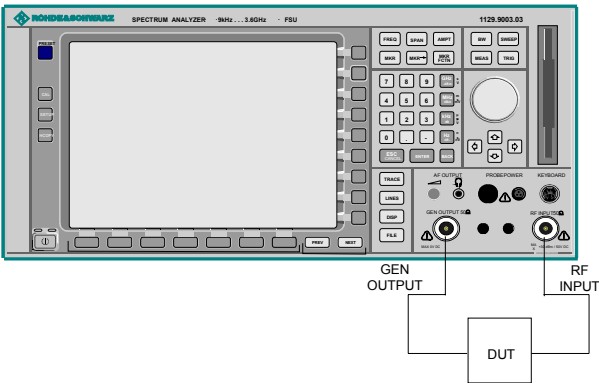
Fig. 4-18 Test setup for transmission measurement
