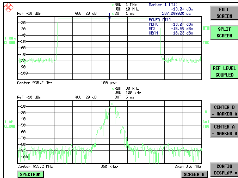
Fig. 4-14 Typical split-screen display, settings are uncoupled
