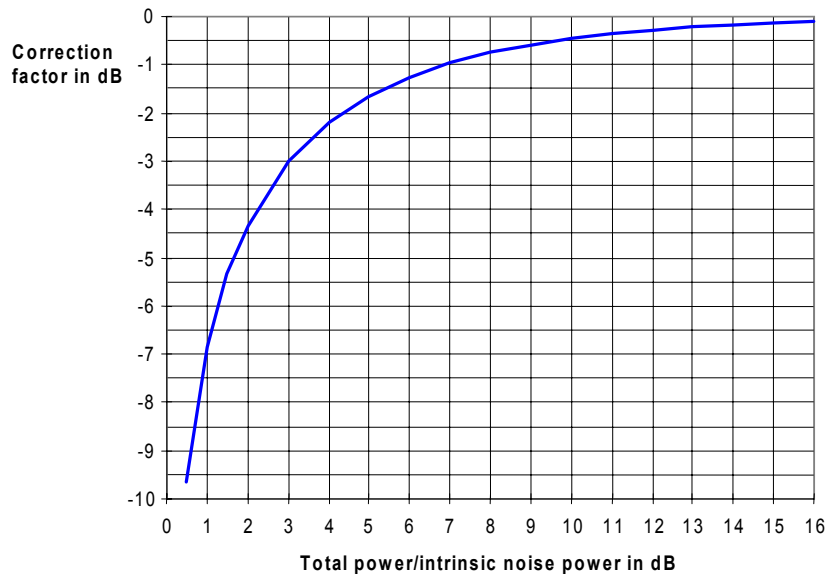
Fig. 2-13 Correction factor for measured noise power as a function of the ratio of total power to the intrinsic noise power of the Spectrum Analyzer.
