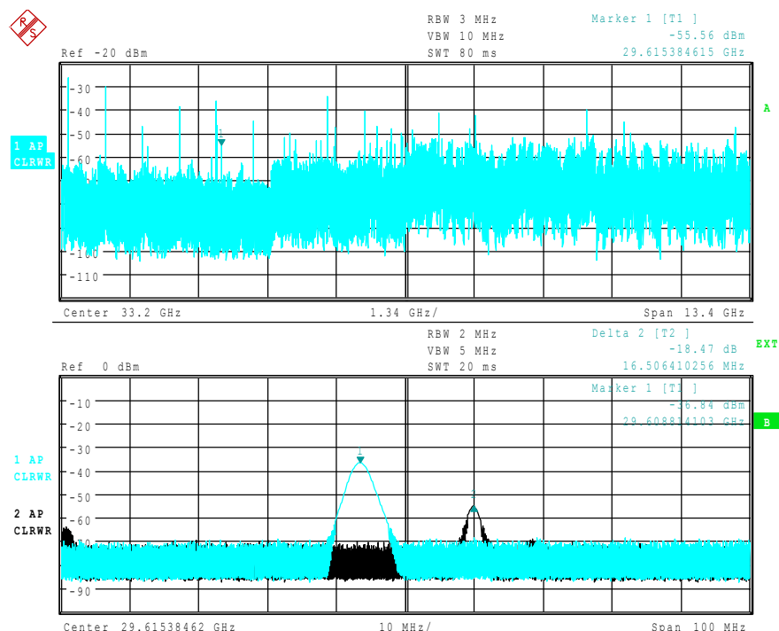
Fig. 4-37 Screen A: Unwanted mixer product not detected by AUTO ID Screen B: Unwanted mixer product not detected by AUTO ID and examined with a small span using SIGNAL ID
