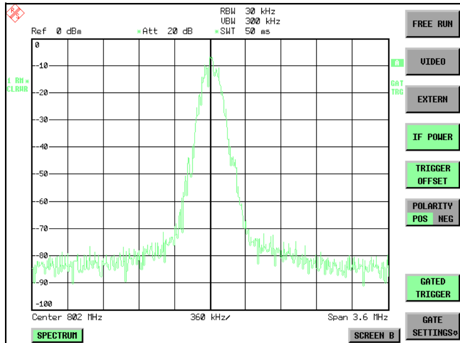
Fig. 4-2 TDMA signal with GATE ON
