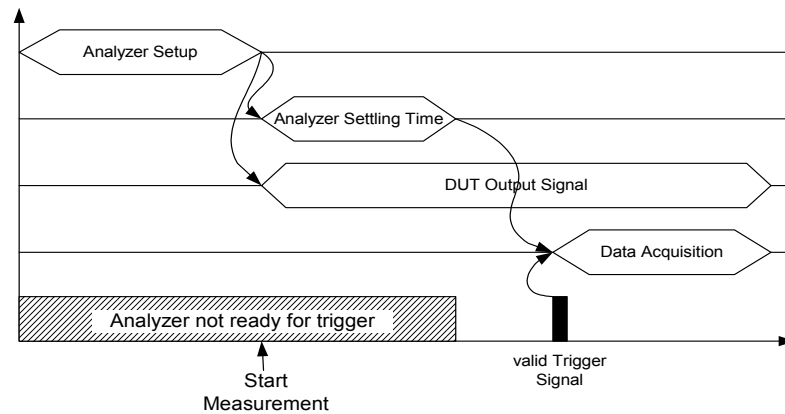
Fig. 4-43 Test with single trigger pulse
