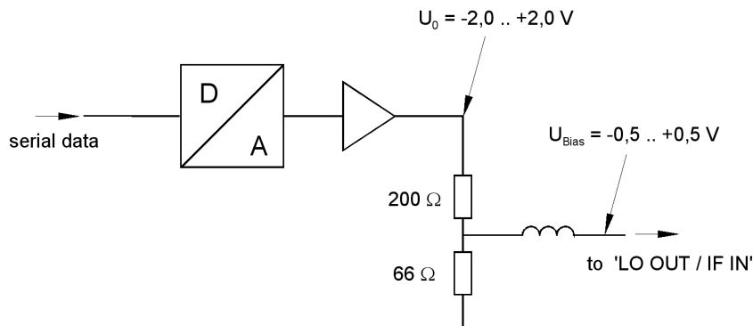
Fig. 4-35 Bias circuit of the Spectrum Analyzer
