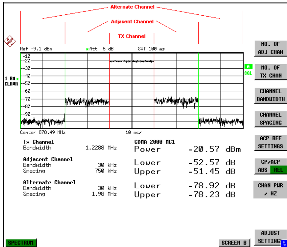
Fig. 4-8 Screen display of adjacent-channel power measurement using the time-domain method
