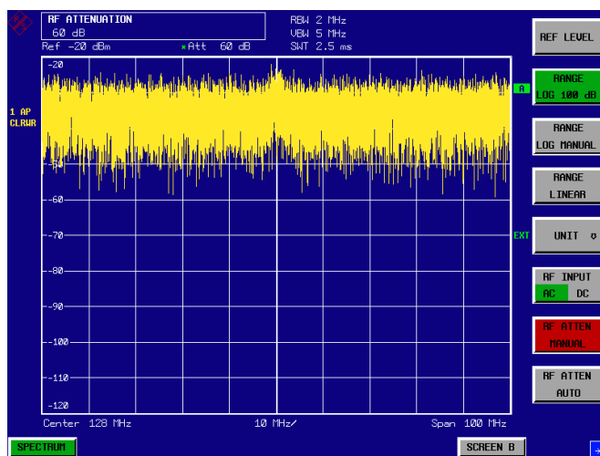
Fig. 2-9 Sinewave signal with low S/N ratio. The signal is measured with the autopeak detector and is completely swamped by the intrinsic noise of the Spectrum Analyzer.
