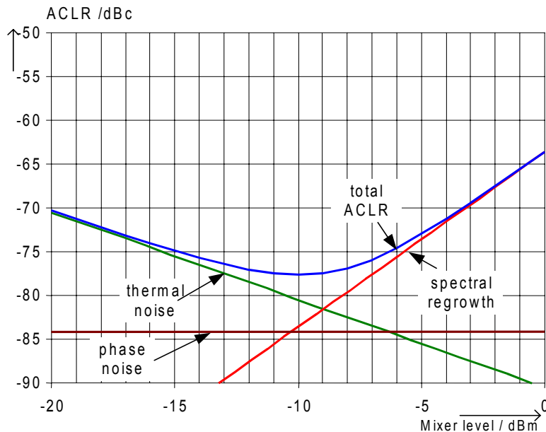
Fig. 2-34 The R&S FSU's dynamic range for adjacent channel power measurements on W-CDMA uplink signals is a function of the mixer level.
