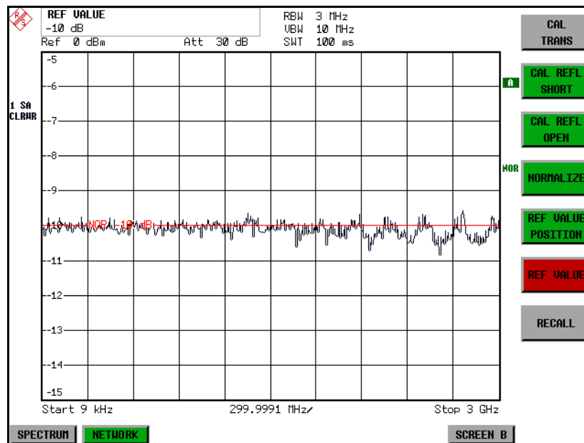
Fig. 4-23 Measurement of a 10dB attenuator pad with 1dB/DIV
