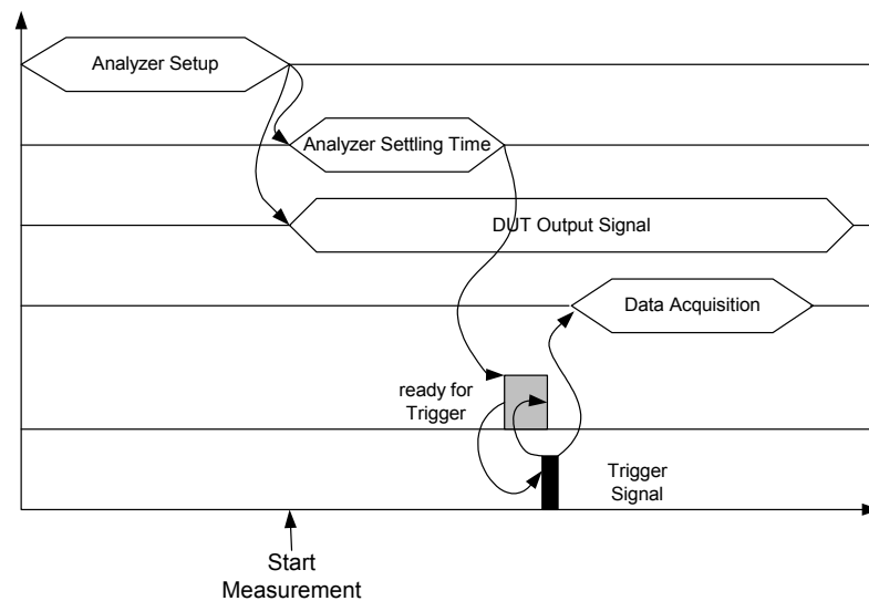
Fig. 4-44 Test with ready-for-trigger signal
