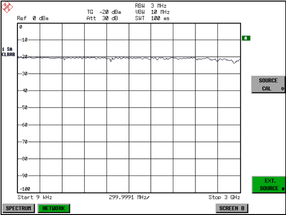
Fig. 4-28 Calibration curve for transmission measurement During the calibration the following message is displayed:
