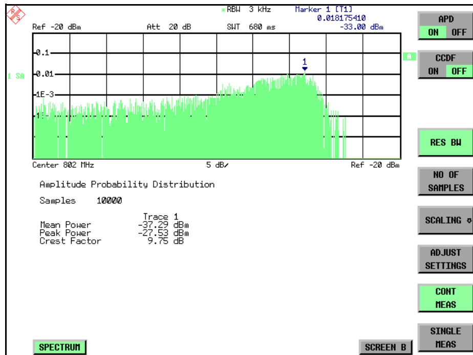
Fig. 4-10 Display of the amplitude probability distribution
