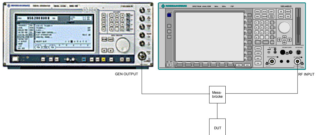
Fig. 4-33 Test setup for reflection measurement
