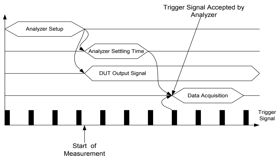
Fig. 4-42 Test with stationary test signal and periodic trigger signal
