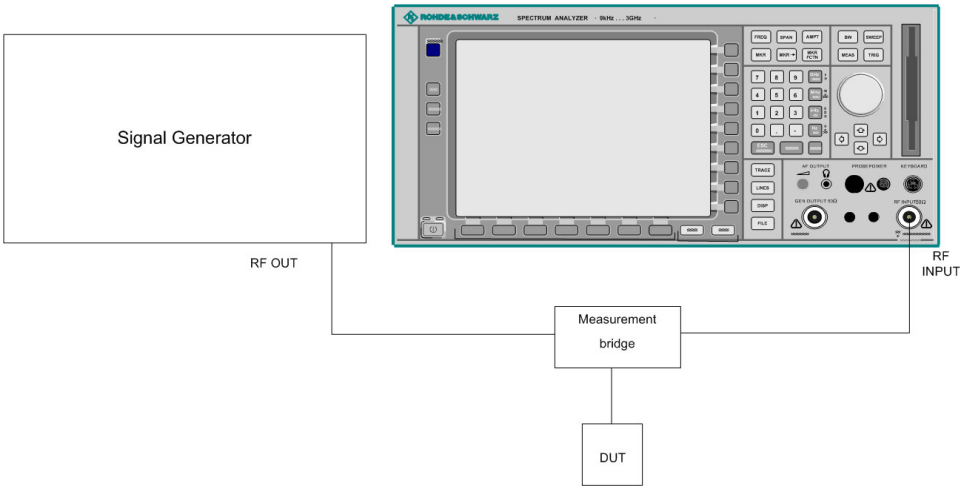
Fig. 4-27 Test setup for transmission measurement
