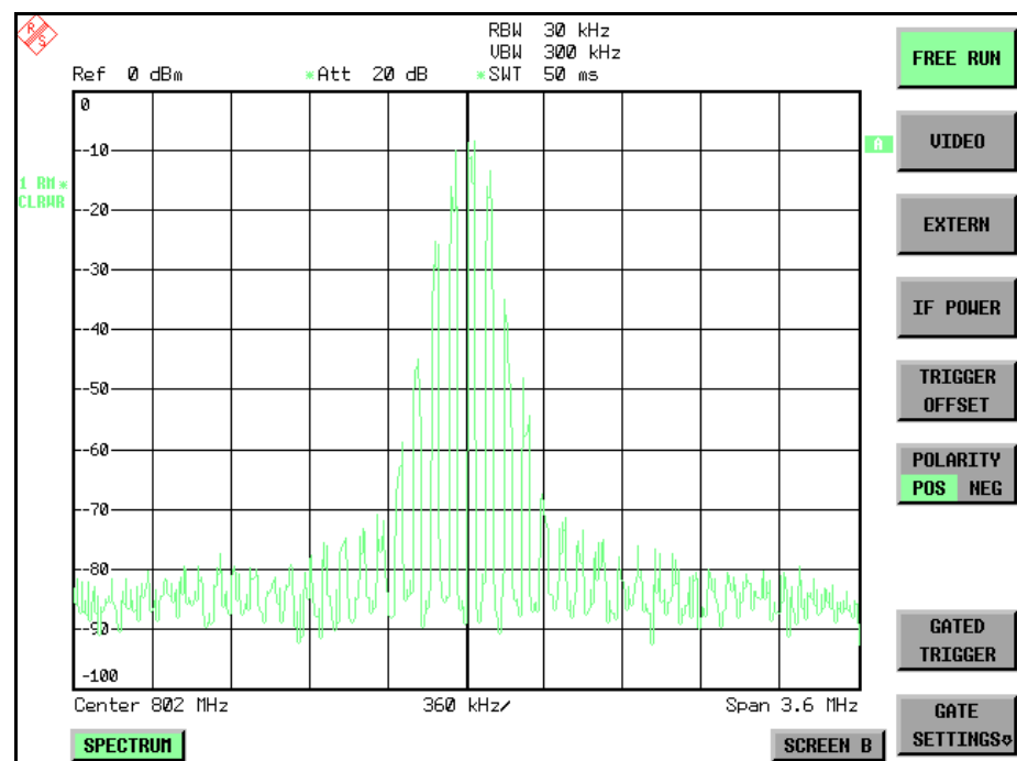
Fig. 4-1 Pulsed signal GATE OFF
