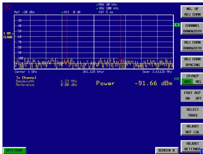
Fig. 2-14 Measurement of the R&S FSU's intrinsic noise power in a 1.23 MHz channel bandwidth.
