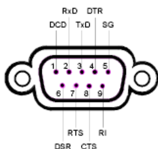
Fig. 8-4 Pin assignment of the RS-232-C interface
