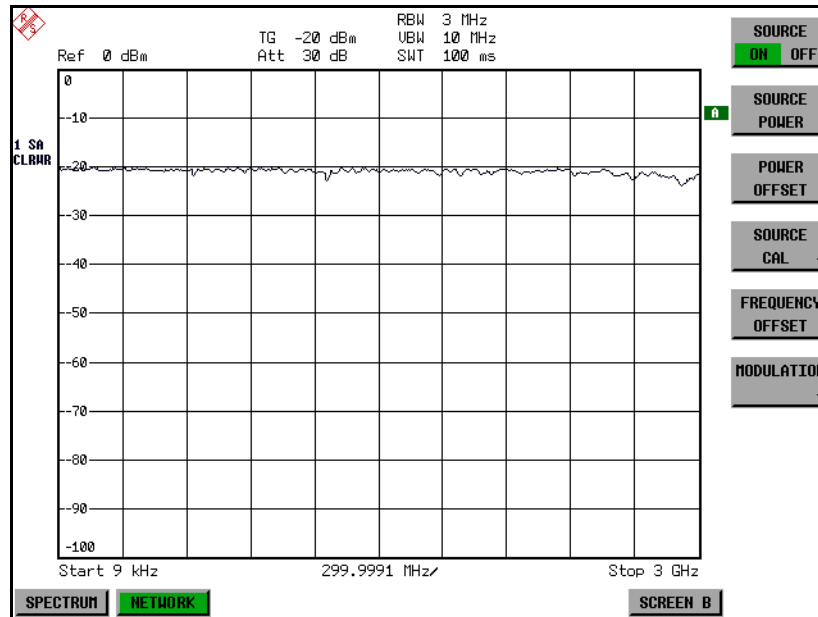
Fig. 4-19 Calibration curve for transmission measurement
