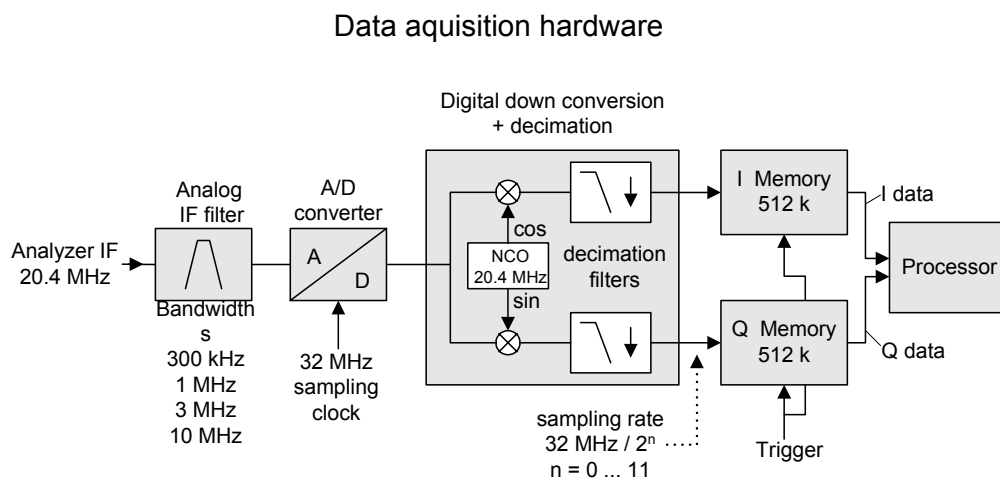
Fig. 7-3 Block diagram illustrating signal processing by the Spectrum Analyzer
