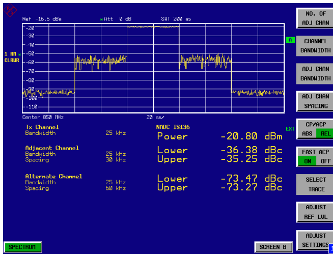
Fig. 2-28 Measuring adjacent channel power in time domain (Fast ACP)
