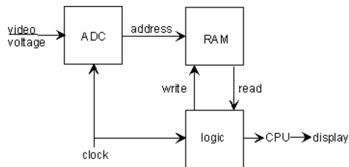
Fig. 4-9 Simplified block diagram for APD measurement
