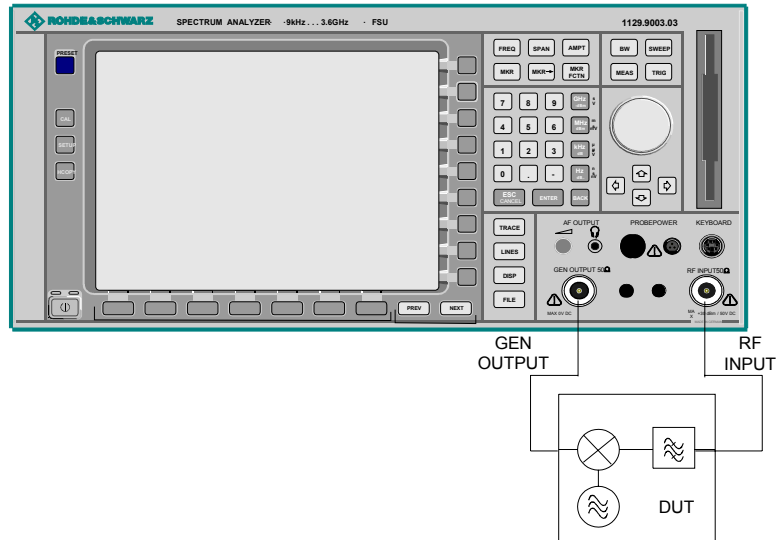
Fig. 4-25 Test setup for frequency converting measurements
