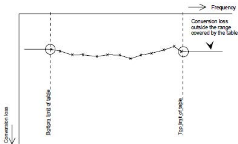
Fig. 3-43: Conversion loss outside the band's frequency range
