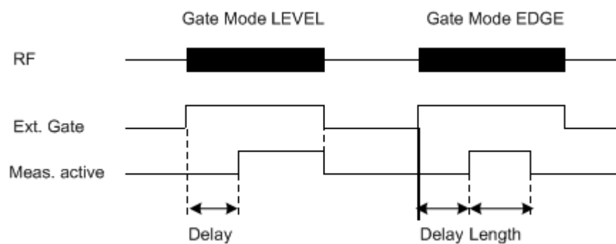
Fig. 5-14: Effects of Gate mode, Gate delay and Gate length
