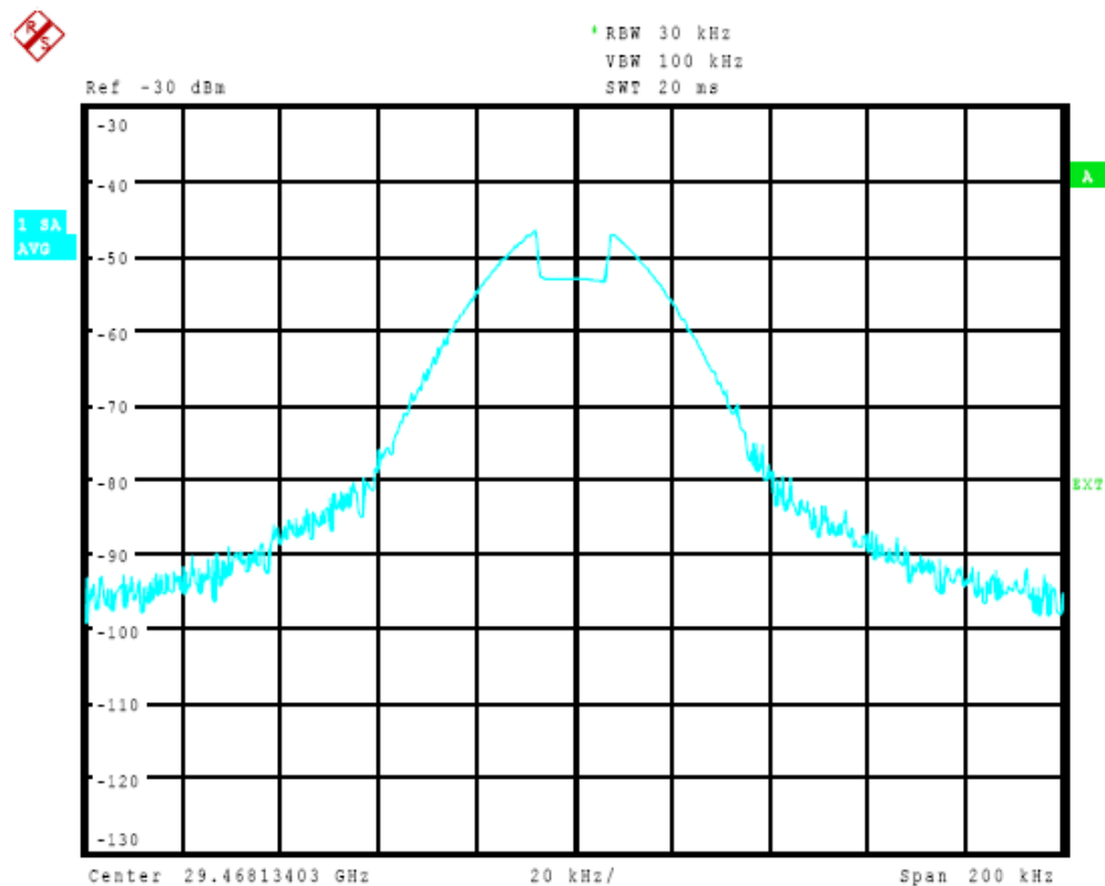
Fig. 5-7: Unwanted mixer products displayed for small span
