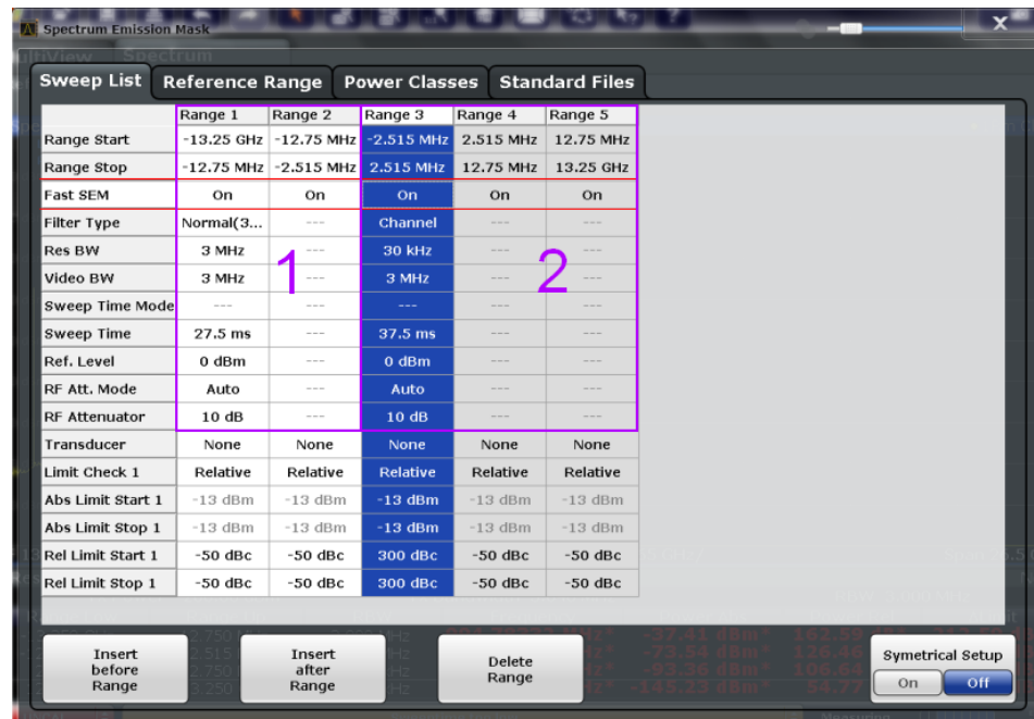
Fig. 4-11: Sweep list using Fast SEM mode
