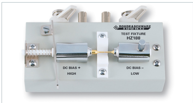
Abb. 8.12: 4-Draht-SMD-Testadapter R&amp;S®HZ188
