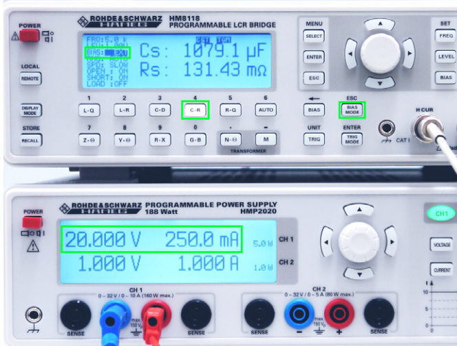
Fig. 7.5: Activate external BIAS preload
