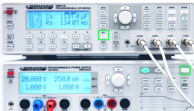
Fig. 7.6: Activate external BIAS preload
