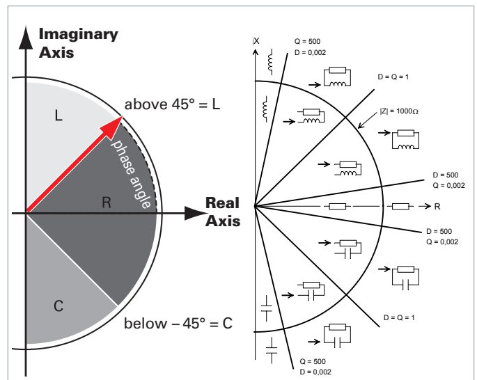
Fig. 3.2: R&S®HM8118 measurement principle, left: schematic, right: detailed presentation.
