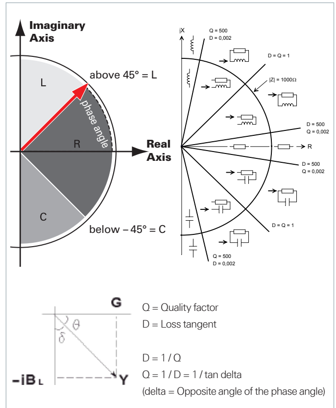
Fig. 4.3: Measurement principle
