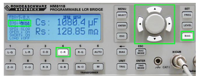
Fig. 7.3: Internal BIAS preload
