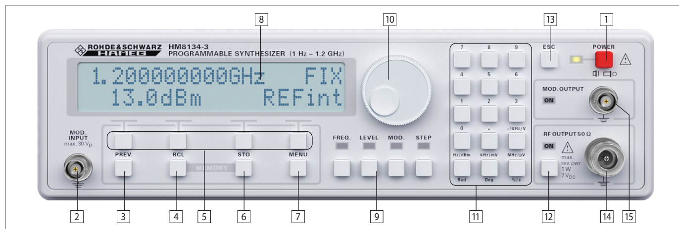
Fig. 2.1: Front panel of the HM8134-3
