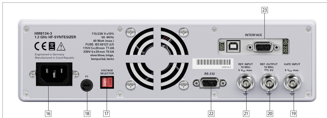
Fig. 2.2: Rear panel of the HM8134-3
