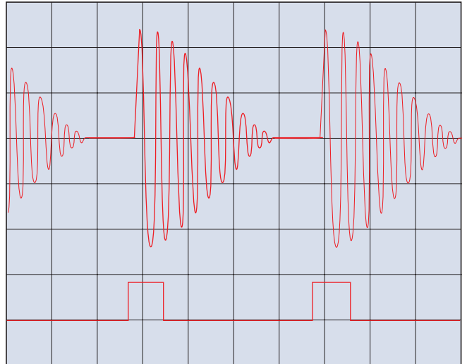
Abb. 4.2: getriggertes Arbitrary-Signal
